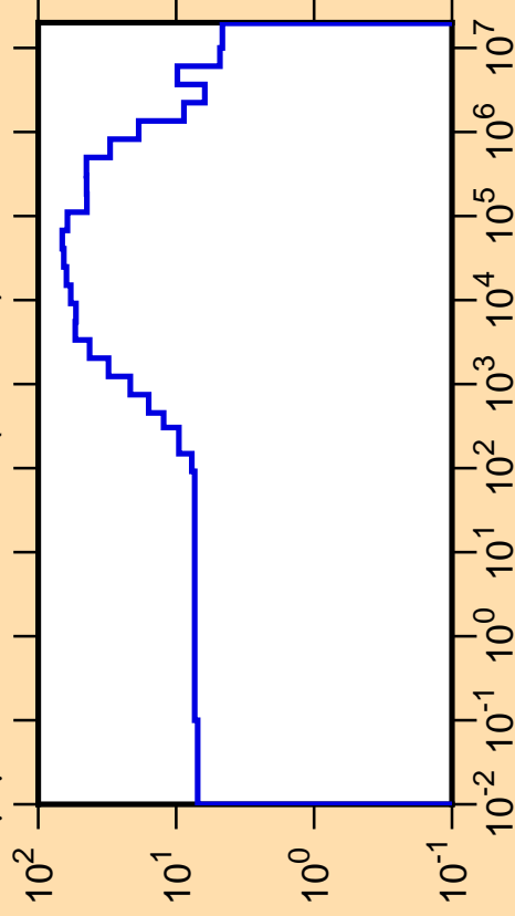
\Delta\mu/\mu vs. E for ^{125}\text{Ba}(\text{mt251})
