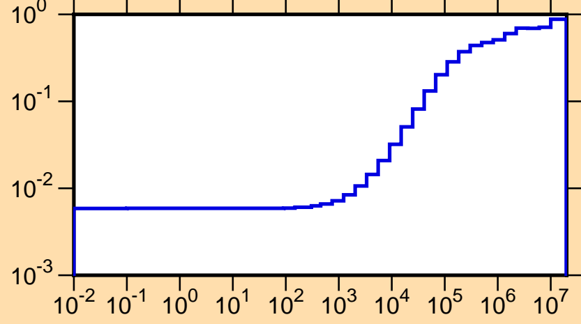
\mu vs. E for ^{125}\text{Ba}(\text{mt251})
