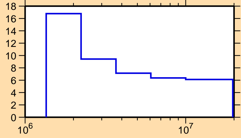
\Delta\sigma/\sigma vs. E for ^{125}\text{Ba}(n,n\text{onel.})
