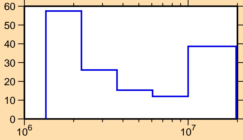
\Delta\sigma/\sigma vs. E for ^{125}\text{Ba}(n,n\text{cont.})
