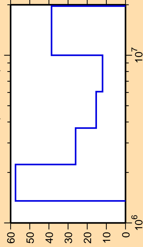
\Delta\sigma/\sigma vs. E for ^{125}\text{Ba}(n,\text{ncont.})
