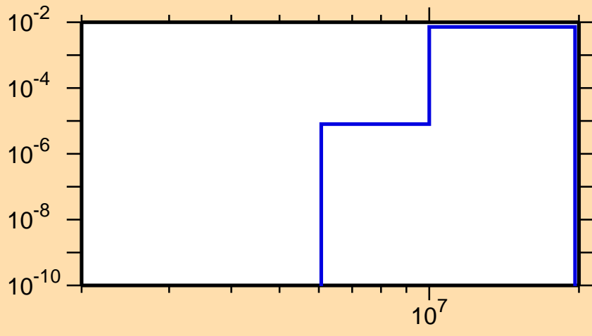
\sigma vs. E for ^{125}\text{Ba}(n,d)
