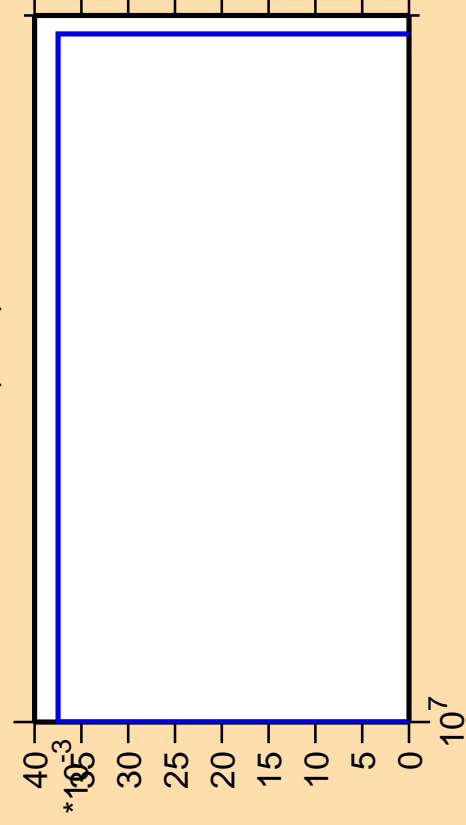
\Delta\sigma/\sigma vs. E for ^{125}\text{Ba}(n,\text{nt})
