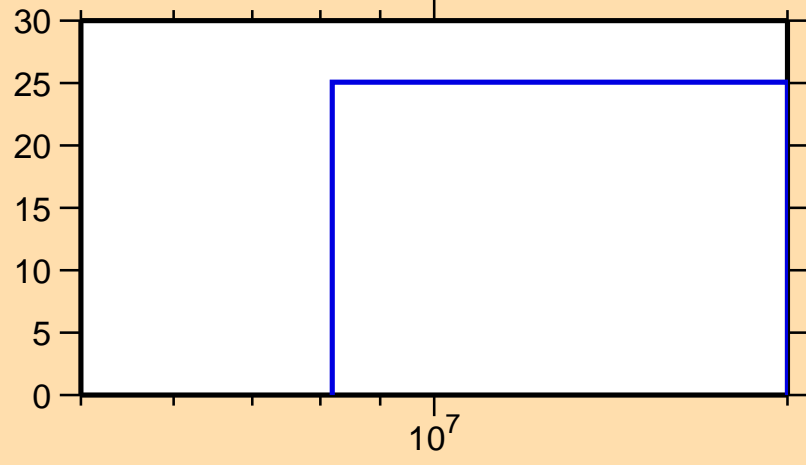
\Delta\sigma/\sigma vs. E for ^{125}\text{Ba}(n,\text{inel.})
