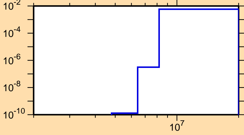
\sigma vs. E for ^{125}\text{Ba}(n,d)
