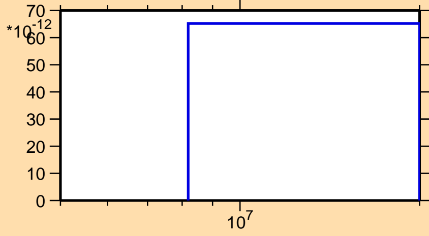
\sigma vs. E for ^{125}\text{Ba}(\text{mt } 45)
