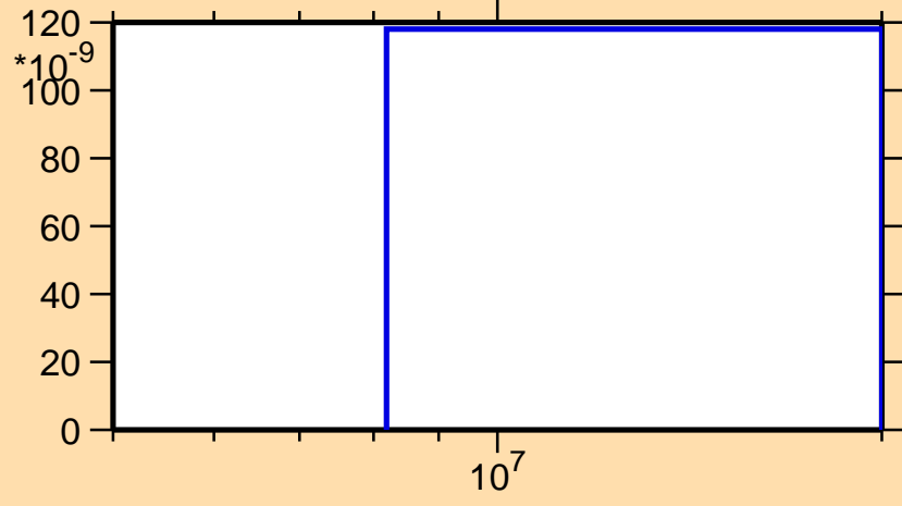
\sigma vs. E for ^{125}\text{Ba}(n,2n\alpha)
