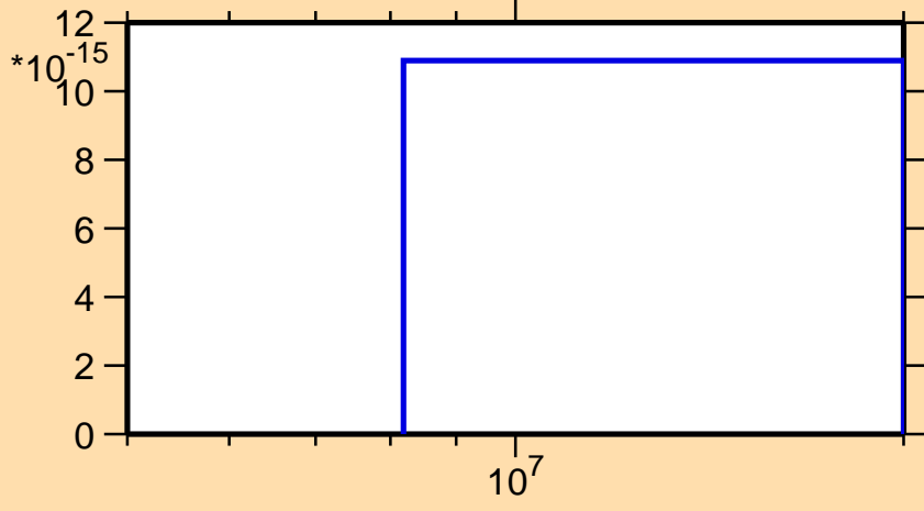
\sigma vs. E for ^{125}\text{Ba}(n,\text{nt})
