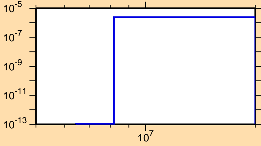
\sigma vs. E for ^{125}\text{Ba}(n,\text{He3})
