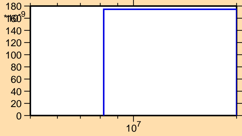
\sigma vs. E for ^{125}\text{Ba}(n,\text{nd})
