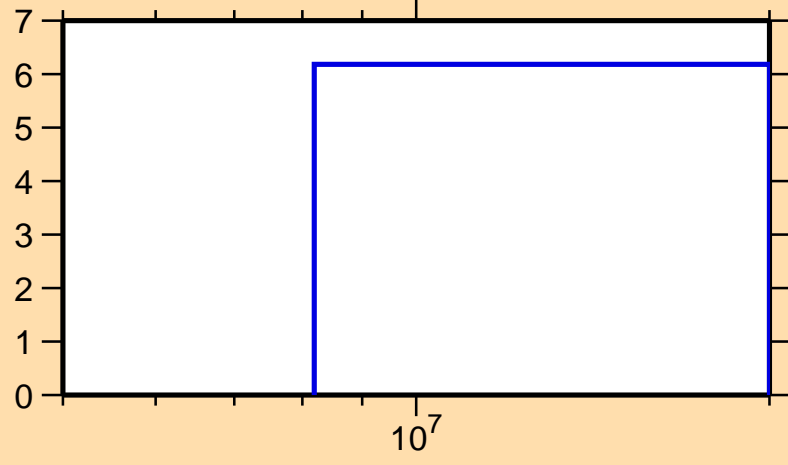
\Delta\sigma/\sigma vs. E for ^{125}\text{Ba}(n,\text{nonel.})
