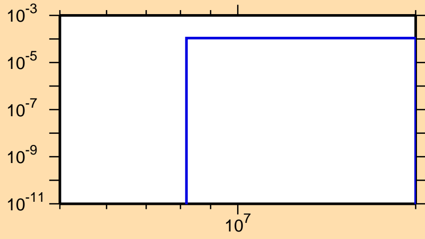
\sigma vs. E for ^{125}\text{Ba}(n,t)
