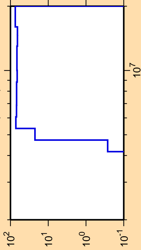
\Delta\sigma/\sigma vs. E for ^{126}\text{Ba}(n,n\alpha)
