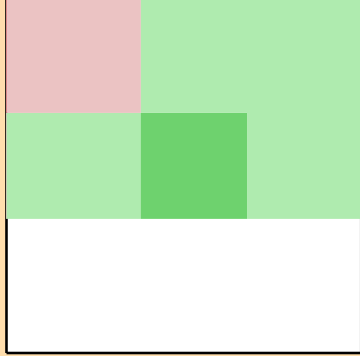
\Delta\sigma/\sigma vs. E for ^{126}\text{Ba}(n,\text{el.})
