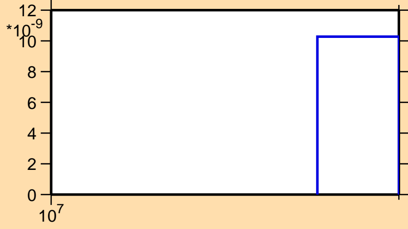
\sigma vs. E for ^{126}\text{Ba}(n,3n)
