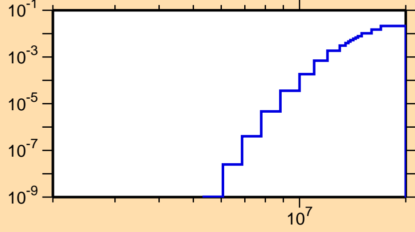
\sigma vs. E for ^{126}\text{Ba}(n,n\alpha)
