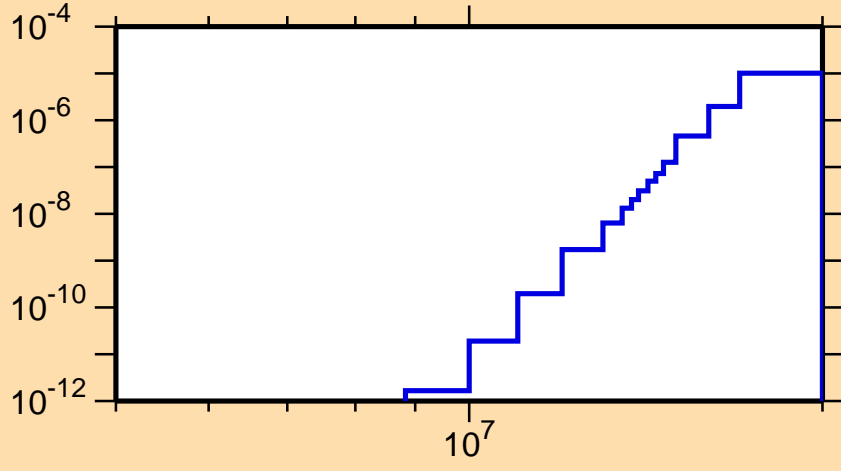
\sigma vs. E for ^{126}\text{Ba}(n,\text{He3})
