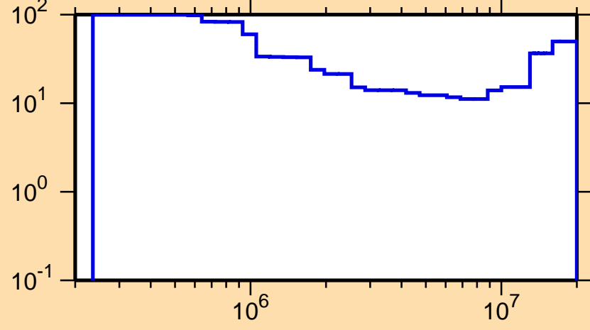
\Delta\sigma/\sigma vs. E for ^{126}\text{Ba}(n,\text{inel.})
