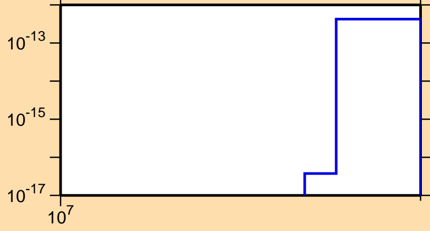
\sigma vs. E for ^{126}\text{Ba} (mt 34)
