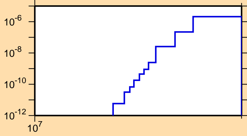
\sigma vs. E for ^{126}\text{Ba}(n,pd)
