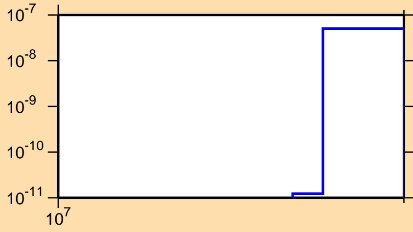
\sigma vs. E for ^{126}\text{Ba}(n,\text{nd})
