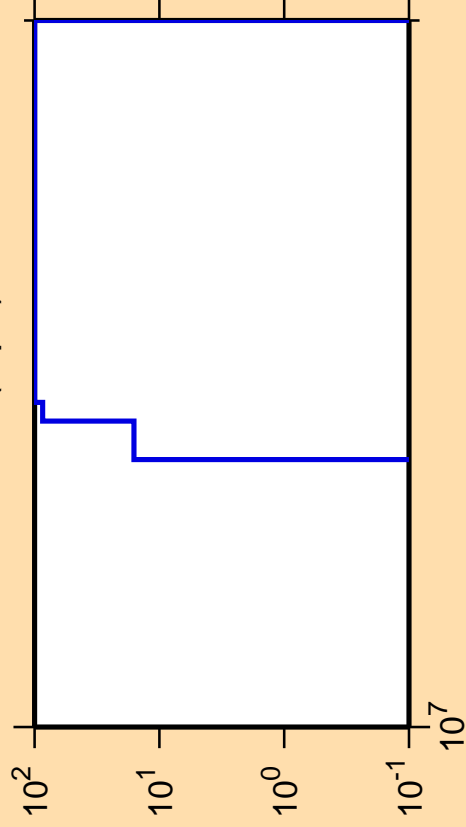
\Delta\sigma/\sigma vs. E for ^{126}\text{Ba}(n,pd)
