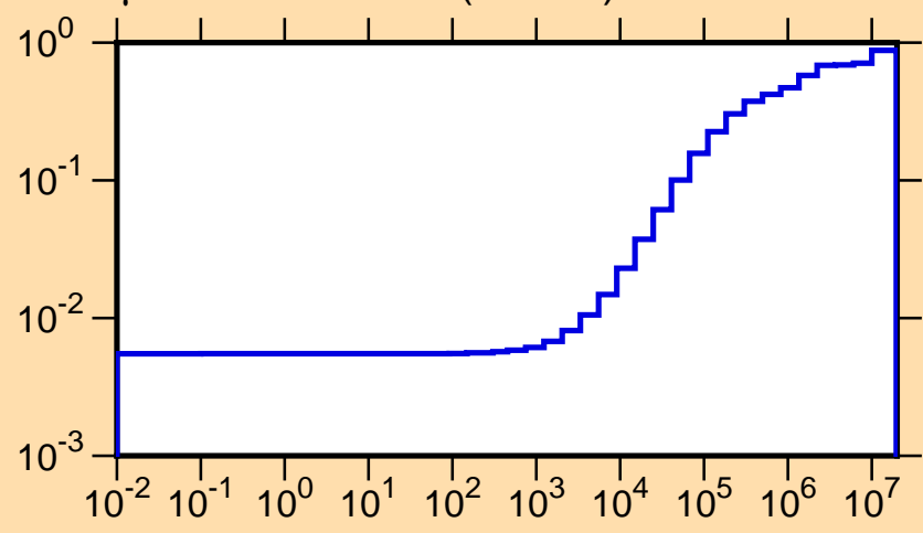
\mu vs. E for ^{126}\text{Ba}(\text{mt251})
