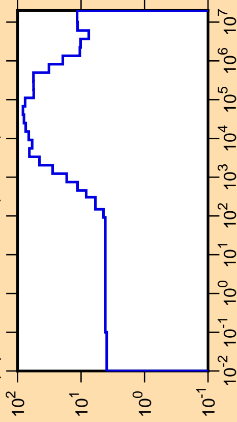
\Delta\mu/\mu vs. E for ^{126}\text{Ba}(\text{mt251})
