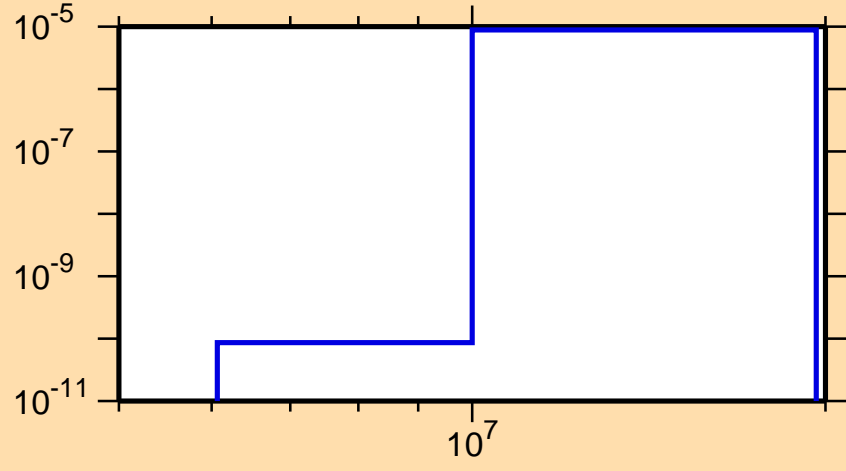
\sigma vs. E for ^{126}\text{Ba}(n,p\alpha)
