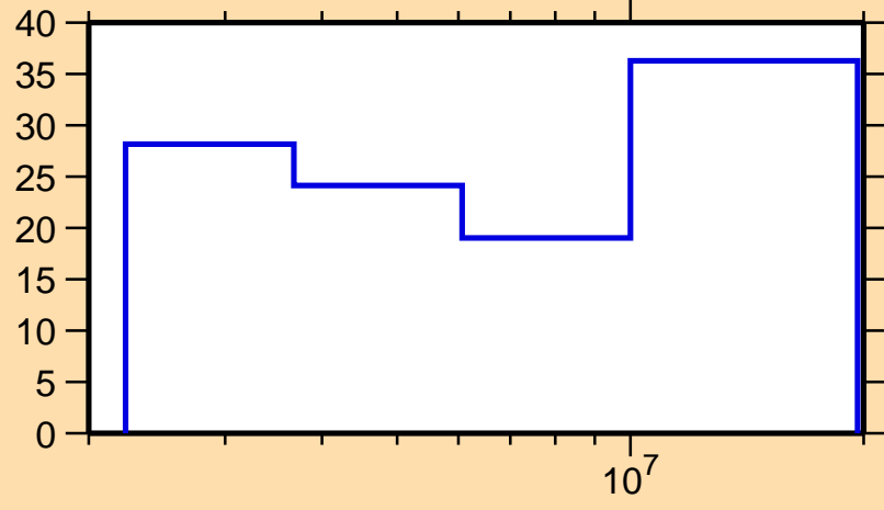
\Delta\sigma/\sigma vs. E for ^{126}\text{Ba}(n,n\text{cont.})
