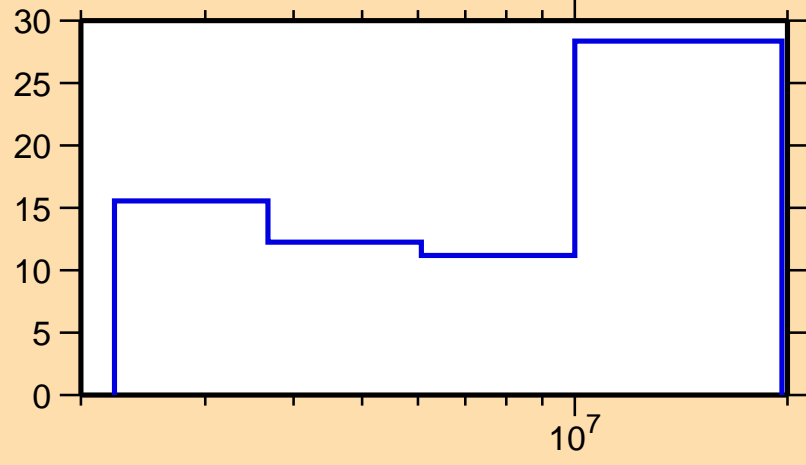
\Delta\sigma/\sigma vs. E for ^{126}\text{Ba}(n,\text{inel.})
