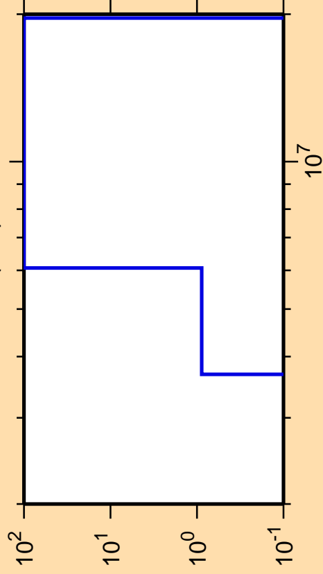
\Delta\sigma/\sigma vs. E for ^{126}\text{Ba}(n,d)
