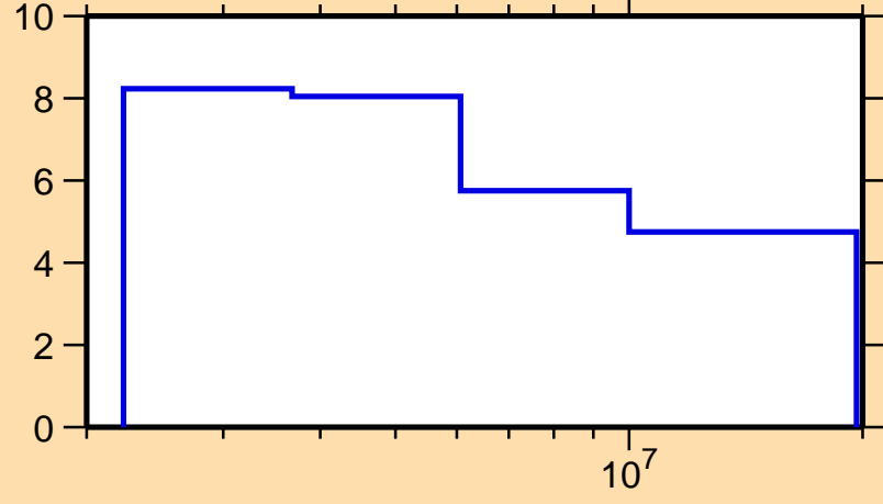
\Delta\sigma/\sigma vs. E for ^{126}\text{Ba}(n,n\text{onel.})
