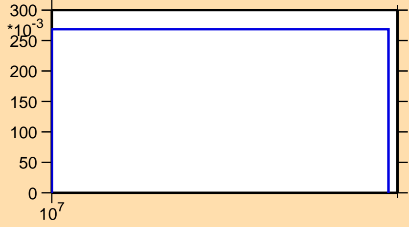
\sigma vs. E for ^{126}\text{Ba}(n,2n)
