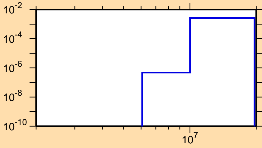
\sigma vs. E for ^{126}\text{Ba}(n,d)
