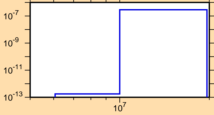
\sigma vs. E for ^{126}\text{Ba}(n,\text{He3})
