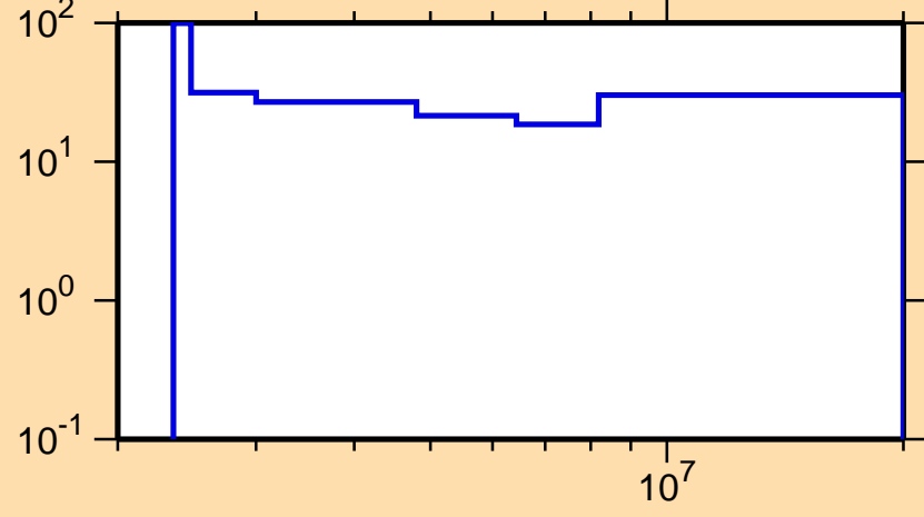
\Delta\sigma/\sigma vs. E for ^{126}\text{Ba}(n,n\text{cont.})
