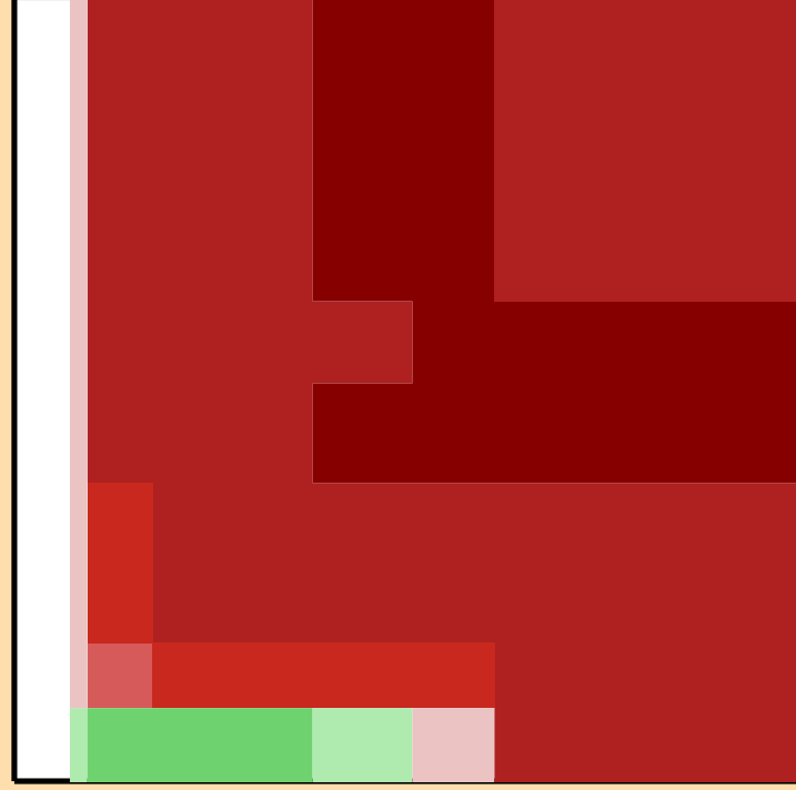
\Delta\sigma/\sigma vs. E for ^{126}\text{Ba}(n,ncont.)
