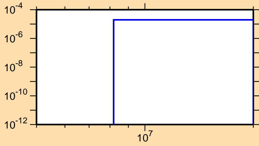
\sigma vs. E for ^{126}\text{Ba}(n,t)
