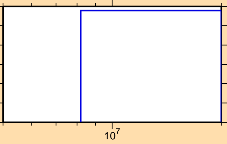
\sigma vs. E for ^{126}\text{Ba}(n,\text{pd})
