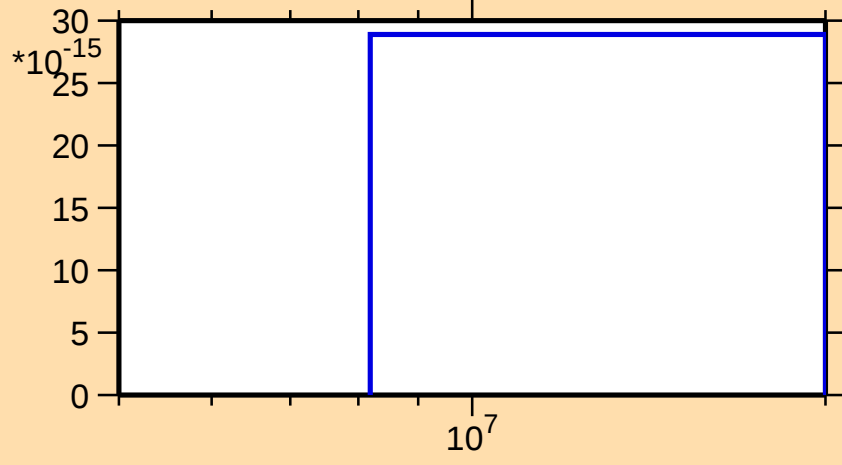
\sigma vs. E for ^{127}\text{Ba}(n,\text{nt})
