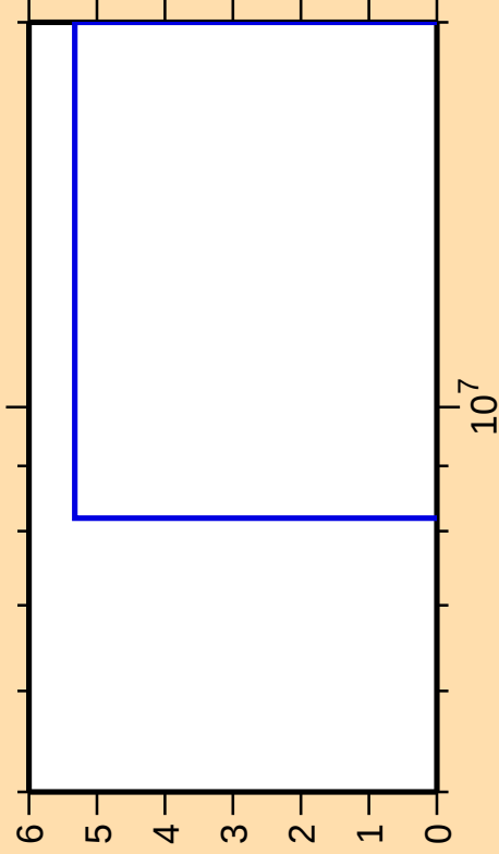
\Delta\sigma/\sigma vs. E for ^{127}\text{Ba}(\text{mt } 45)
