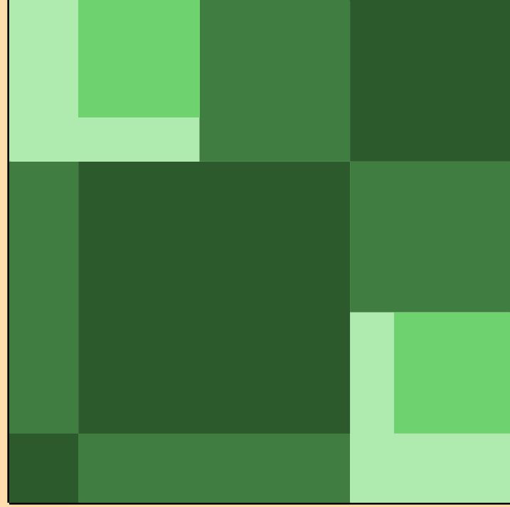
\sigma vs. E for ^{128}\text{Ba}(n,2n)
