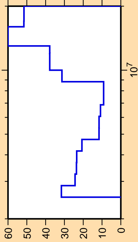
\Delta\sigma/\sigma vs. E for ^{128}\text{Ba}(n,ncont.)
