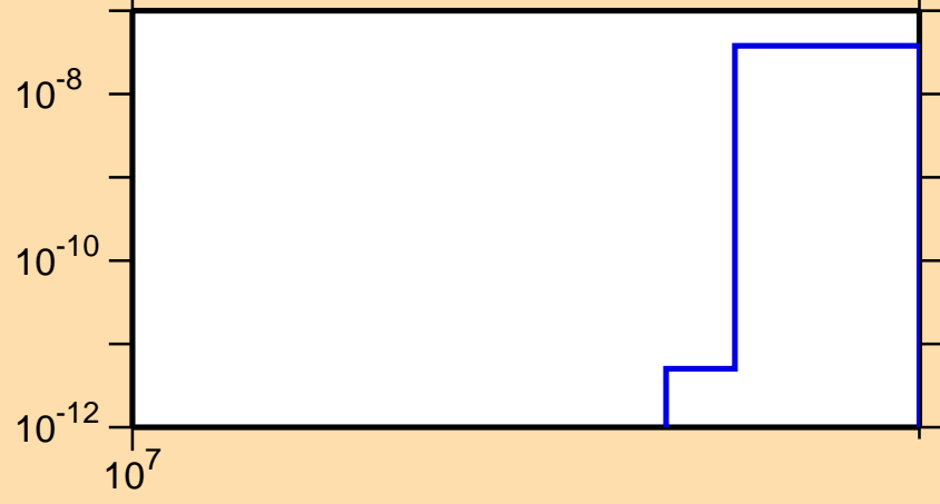
\sigma vs. E for ^{128}\text{Ba}(n,\text{nd})
