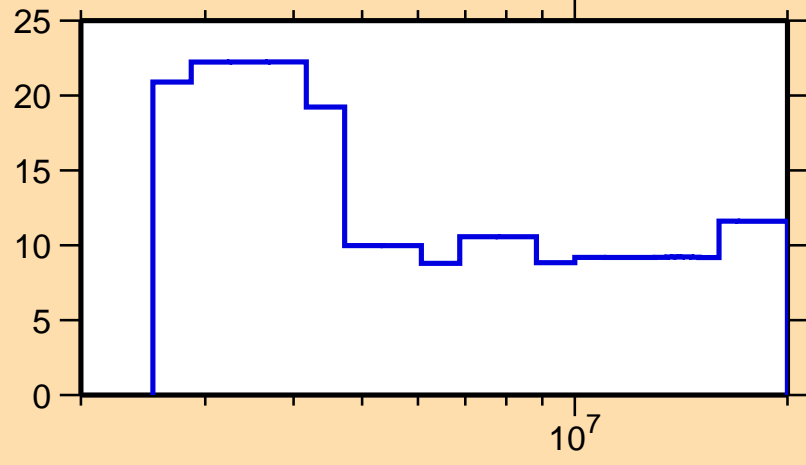
\Delta\sigma/\sigma vs. E for ^{128}\text{Ba}(n,el.)
