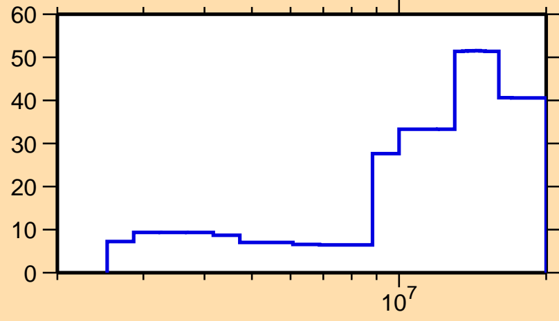
\Delta\sigma/\sigma vs. E for ^{128}\text{Ba}(n,inel.)
