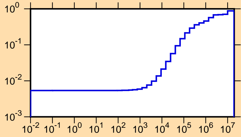
\mu vs. E for ^{128}\text{Ba}(\text{mt251})
