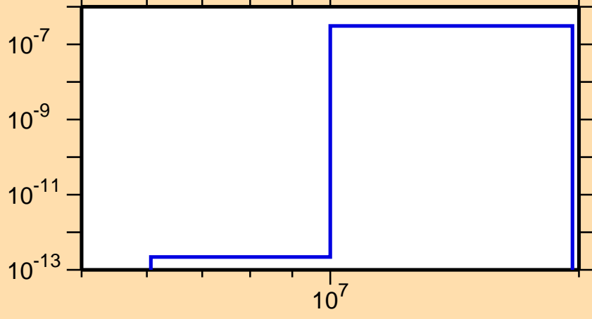
\sigma vs. E for ^{128}\text{Ba}(n,p\alpha)
