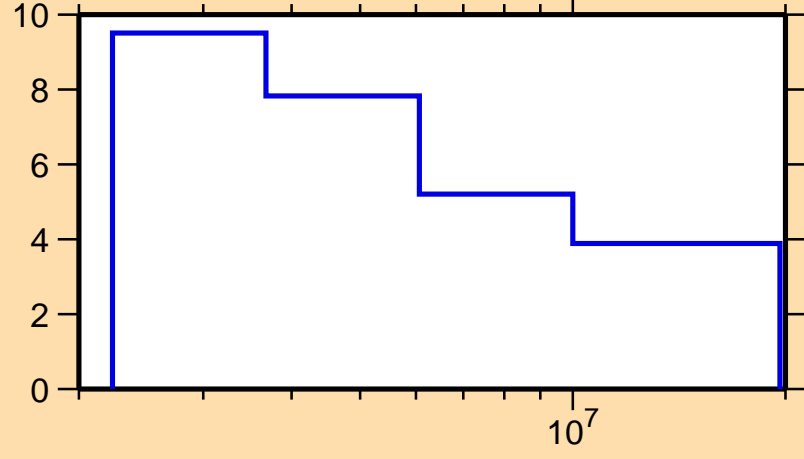
\Delta\sigma/\sigma vs. E for ^{128}\text{Ba}(n,n\text{onel.})
