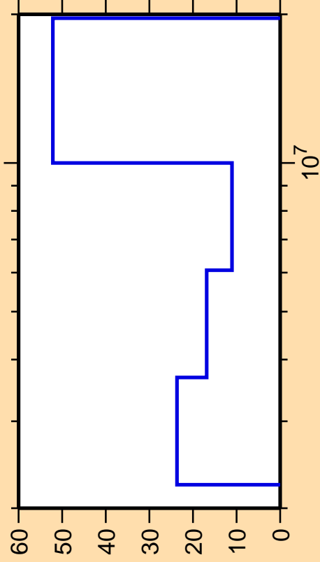
\Delta\sigma/\sigma vs. E for ^{128}\text{Ba}(n,\text{ncont.})
