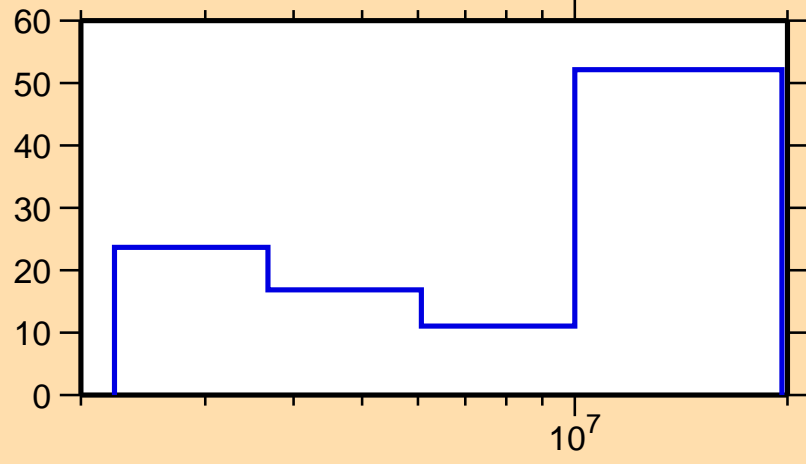
\Delta\sigma/\sigma vs. E for ^{128}\text{Ba}(n,n\text{cont.})
