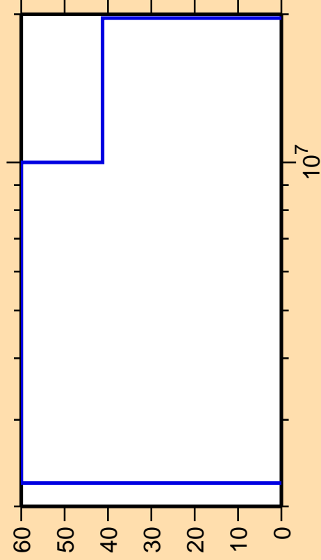
\Delta\sigma/\sigma vs. E for ^{128}\text{Ba}(n,p)
