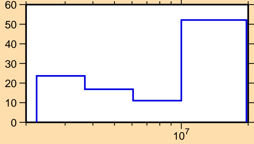
\Delta\sigma/\sigma vs. E for ^{128}\text{Ba}(n,ncont.)
