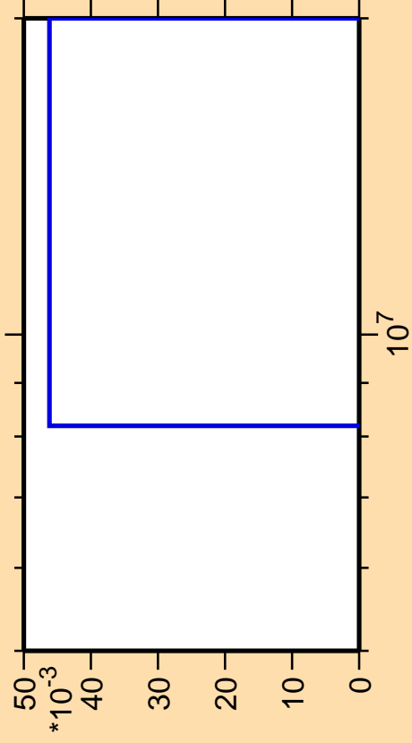
\Delta\sigma/\sigma vs. E for ^{128}\text{Ba}(n,\text{nt})
