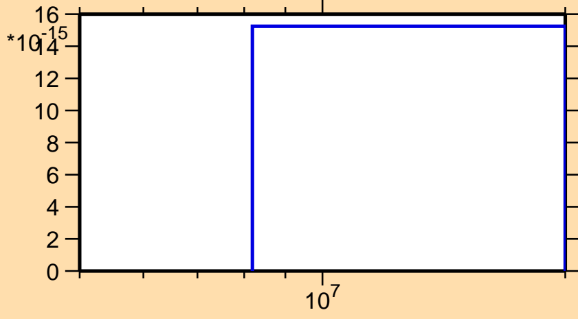
\sigma vs. E for ^{128}\text{Ba}(n,\text{nt})
