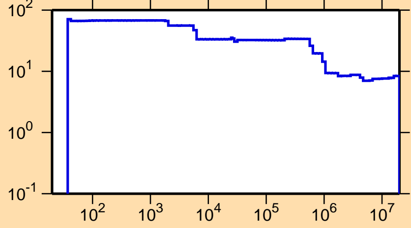
\Delta\sigma/\sigma vs. E for ^{129}\text{Ba}(n,\text{nonel.})
