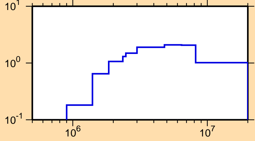
\sigma vs. E for ^{129}\text{Ba}(n,n\text{cont.})
