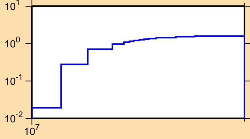
\sigma vs. E for ^{130}\text{Ba}(n,2n)
