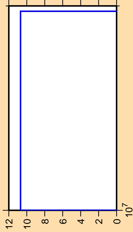
\Delta\sigma/\sigma vs. E for ^{130}\text{Ba}(n,2n)
