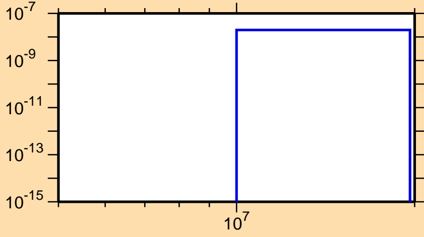
\sigma vs. E for ^{130}\text{Ba}(n,\text{He3})
