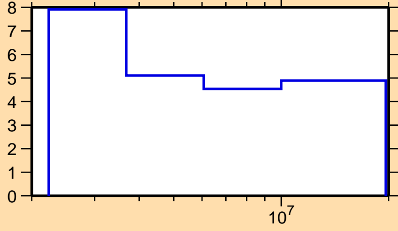
\Delta\sigma/\sigma vs. E for ^{130}\text{Ba}(n,n\text{nonel.})
