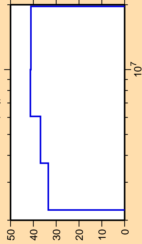
\Delta\sigma/\sigma vs. E for ^{130}\text{Ba}(n,\gamma)
