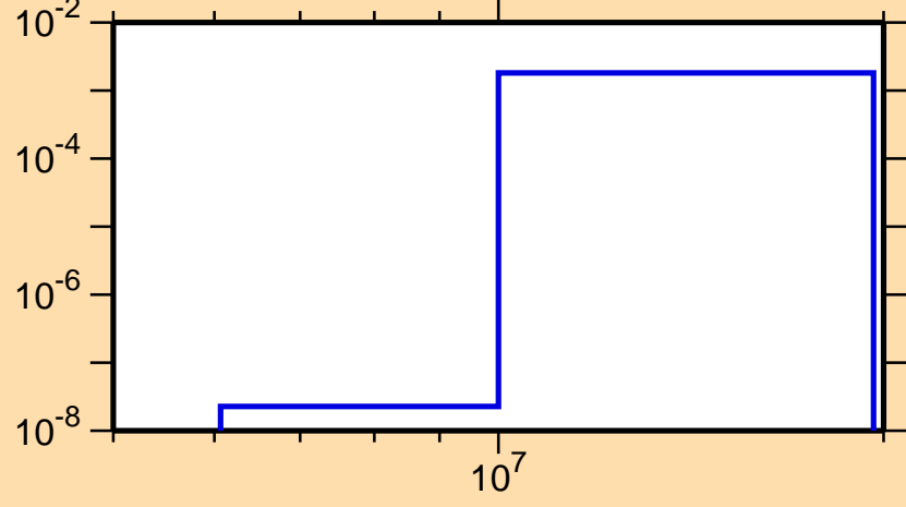
\sigma vs. E for ^{130}\text{Ba}(n,d)
