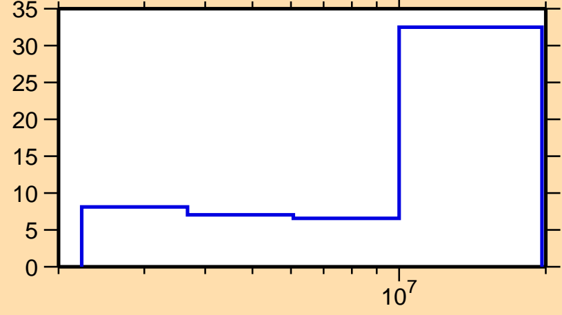
\Delta\sigma/\sigma vs. E for ^{130}\text{Ba}(n,n\text{cont.})
