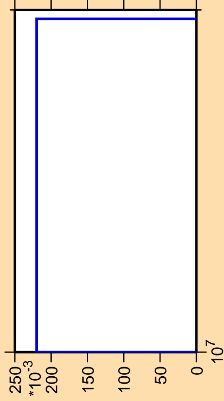
\Delta\sigma/\sigma vs. E for ^{130}\text{Ba}(n,nt)
