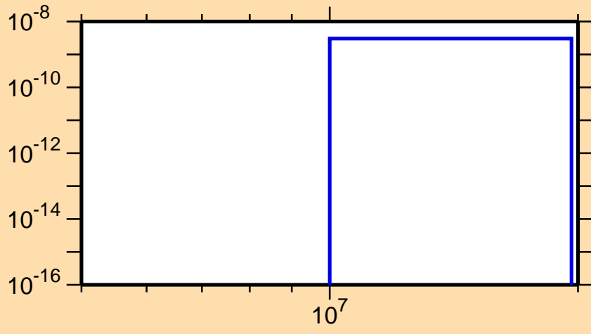
\sigma vs. E for ^{130}\text{Ba}(n,p\alpha)
