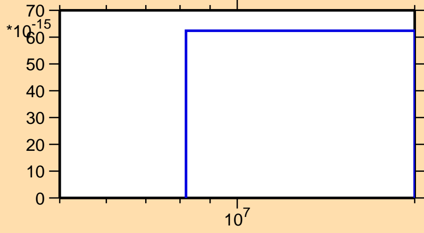
\sigma vs. E for ^{130}\text{Ba}(n,\text{nt})
