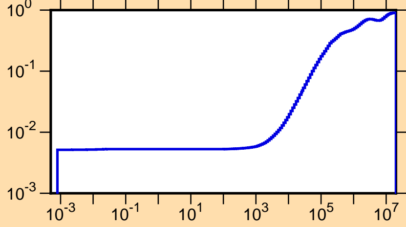
\mu vs. E for ^{131}\text{Ba}(\text{mt251})
