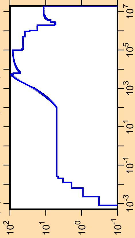
\Delta\mu/\mu vs. E for ^{131}\text{Ba}(\text{mt251})
