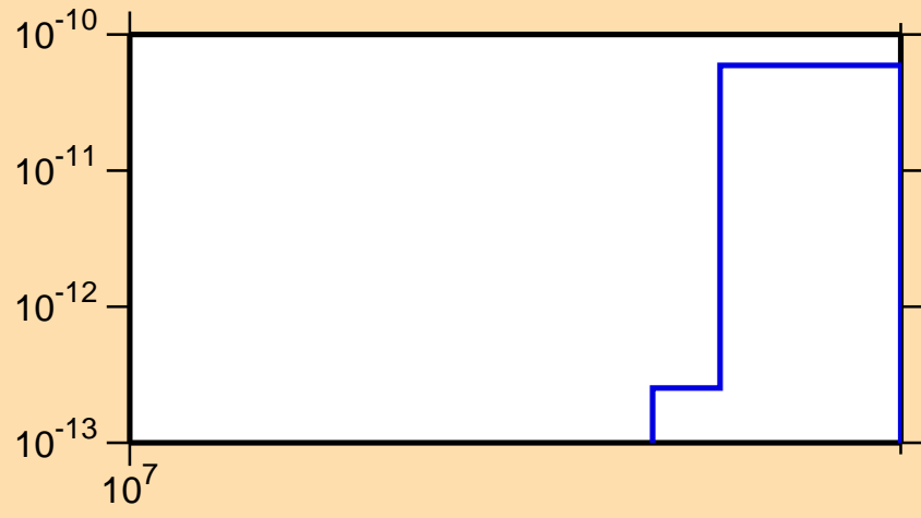
\sigma vs. E for ^{131}\text{Ba}(n,\text{pd})
