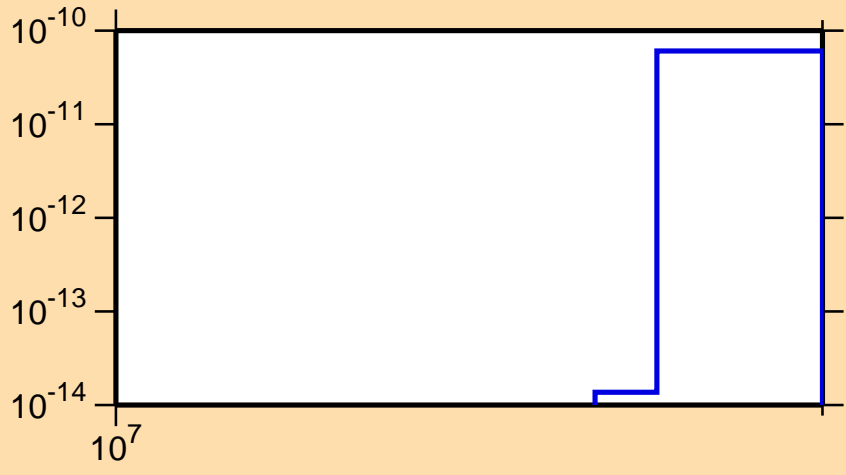
\sigma vs. E for ^{131}\text{Ba}(n,\text{pt})
