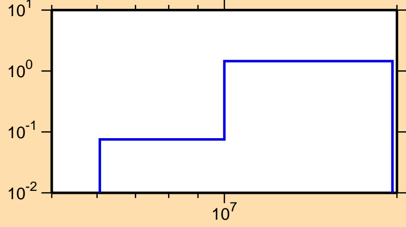
\sigma vs. E for ^{131}\text{Ba}(n,2n)
