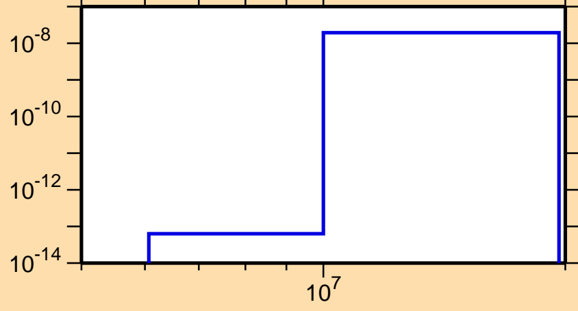
\sigma vs. E for ^{131}\text{Ba}(n,p\alpha)
