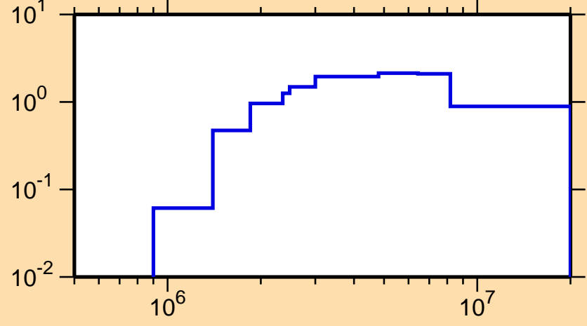
\sigma vs. E for ^{131}\text{Ba}(n,n\text{cont.})
