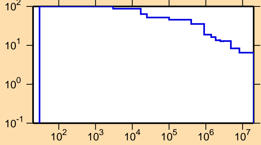
\Delta\sigma/\sigma vs. E for ^{131}\text{Ba}(n,\text{nonel.})
