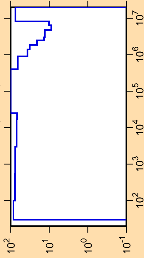
\Delta\sigma/\sigma vs. E for ^{131}\text{Ba}(n,\text{inel.})
