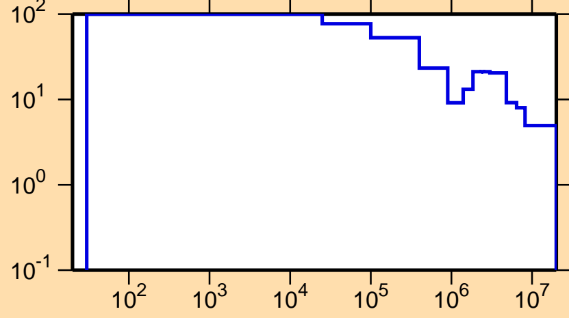
\Delta\sigma/\sigma vs. E for ^{131}\text{Ba}(n,\text{el.})
