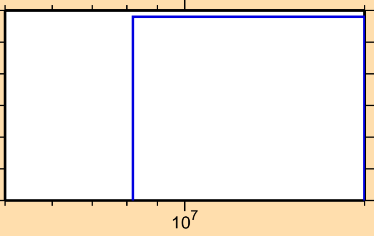
\sigma vs. E for ^{131}\text{Ba}(n,3n)
