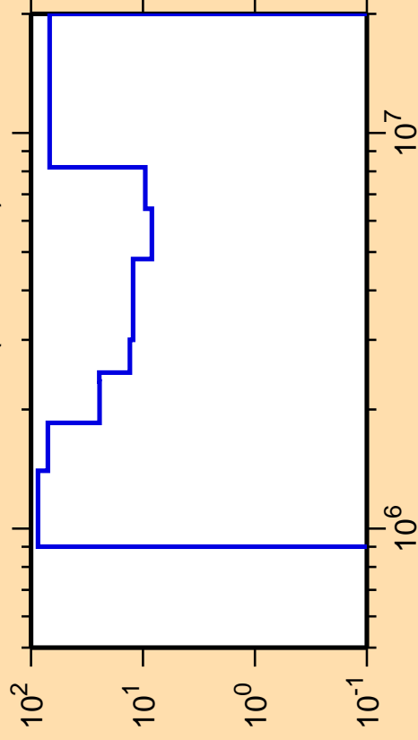
\Delta\sigma/\sigma vs. E for ^{131}\text{Ba}(n,\text{ncont.})
