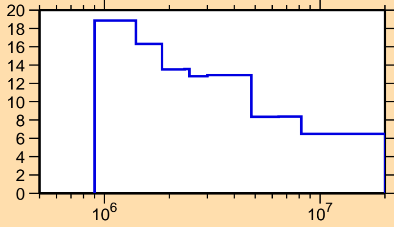
\Delta\sigma/\sigma vs. E for ^{131}\text{Ba}(n,n\text{nonel.})
