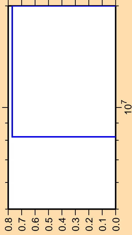
\Delta\sigma/\sigma vs. E for ^{131}\text{Ba}(n,nt)
