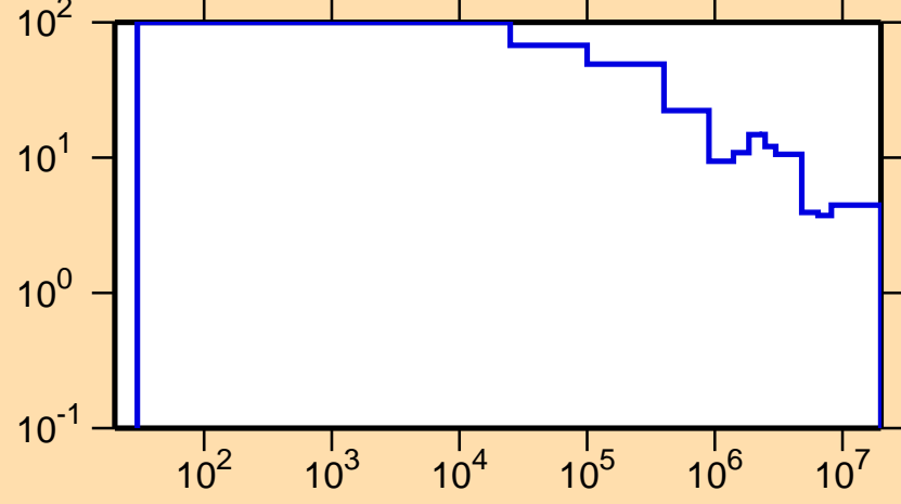
\Delta\sigma/\sigma vs. E for ^{131}\text{Ba}(n,\text{tot.})
