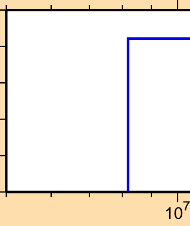
\sigma vs. E for ^{131}\text{Ba}(n,\text{nd})
