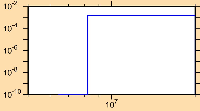
\sigma vs. E for ^{131}\text{Ba}(n,d)
