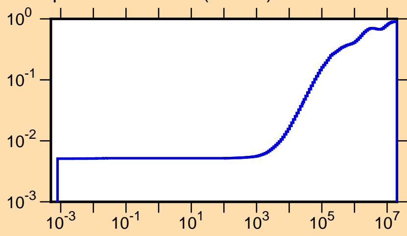
\mu vs. E for ^{132}\text{Ba}(\text{mt251})
