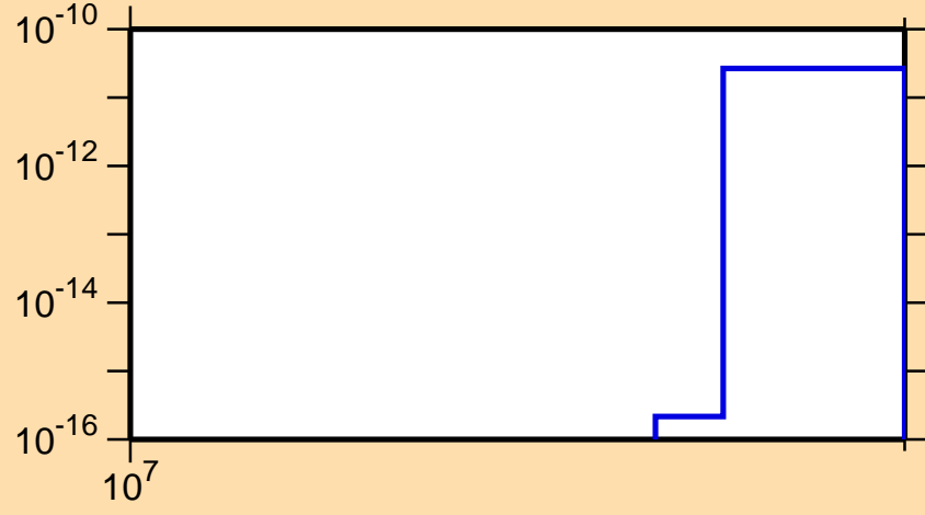
\sigma vs. E for ^{132}\text{Ba}(n,nt)
