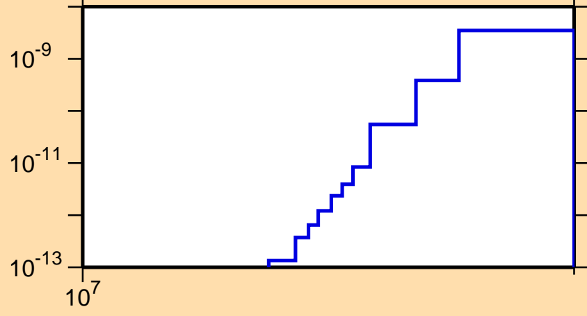
\sigma vs. E for ^{132}\text{Ba}(n,p\alpha)
