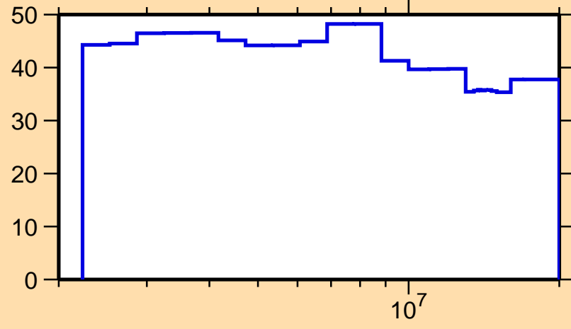
\Delta\sigma/\sigma vs. E for ^{132}\text{Ba}(n,n_1)
