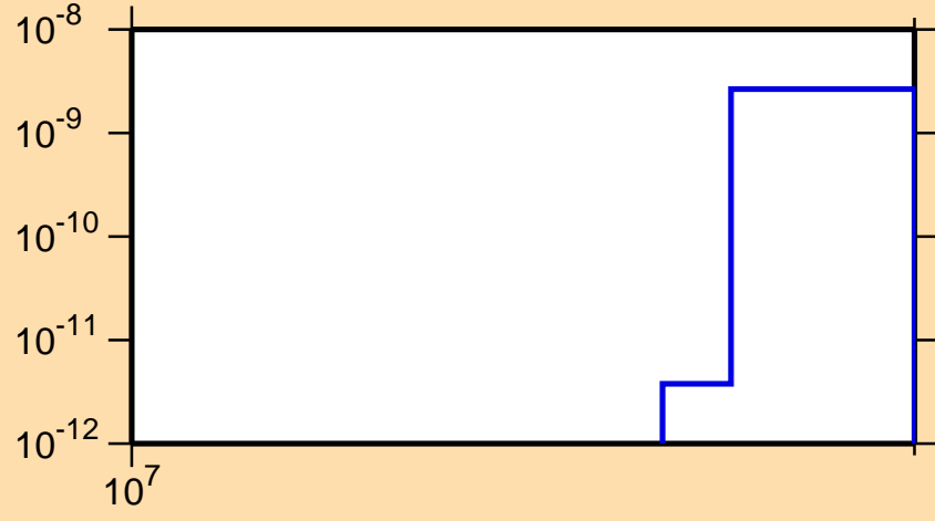
\sigma vs. E for ^{132}\text{Ba}(n,2n\alpha)
