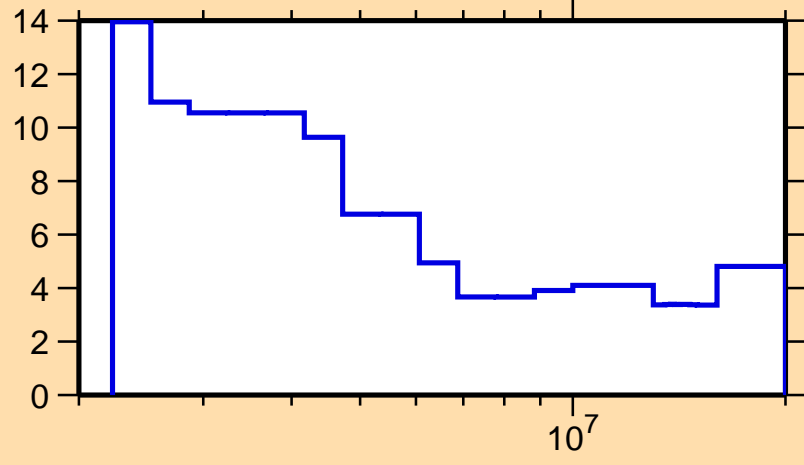
\Delta\sigma/\sigma vs. E for ^{132}\text{Ba}(n,\text{tot.})
