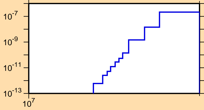
\sigma vs. E for ^{132}\text{Ba}(n,\text{He3})
