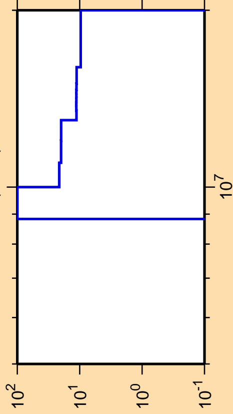
\Delta\sigma/\sigma vs. E for ^{132}\text{Ba}(n,2n)
