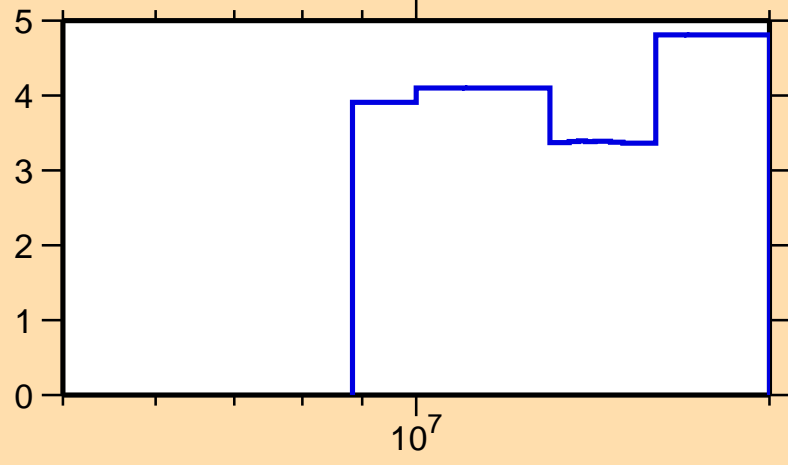
\Delta\sigma/\sigma vs. E for ^{132}\text{Ba}(n,\text{tot.})
