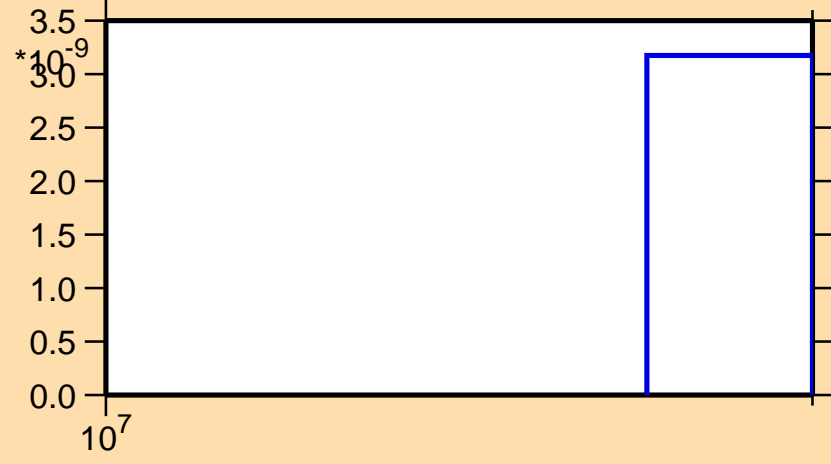
\sigma vs. E for ^{132}\text{Ba}(n,2np)
