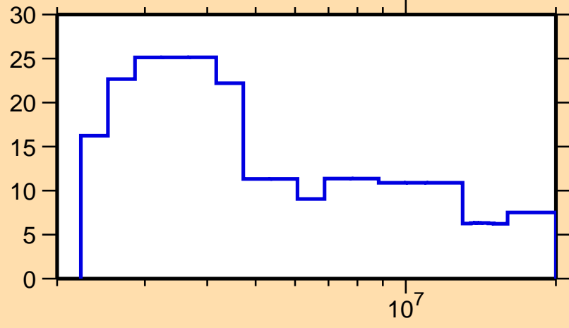
\Delta\sigma/\sigma vs. E for ^{132}\text{Ba}(n,\text{el.})
