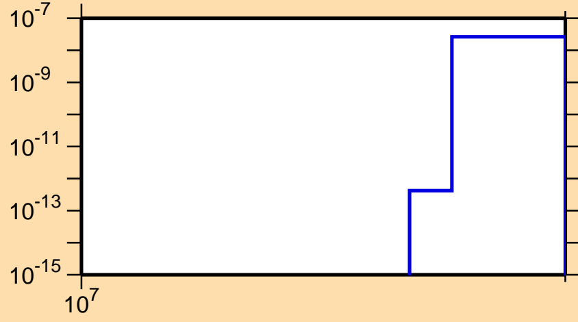
\sigma vs. E for ^{132}\text{Ba}(n,\text{nd})
