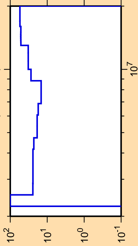
\Delta\sigma/\sigma vs. E for ^{132}\text{Ba}(n,\text{ncont.})
