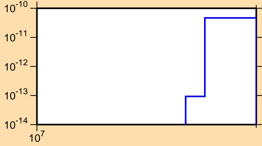
\sigma vs. E for ^{132}\text{Ba}(n,pd)
