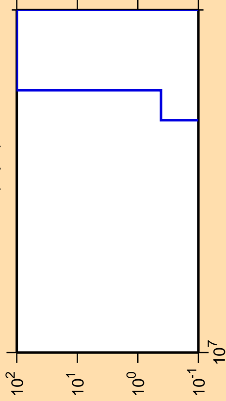
\Delta\sigma/\sigma vs. E for ^{132}\text{Ba}(n,pd)
