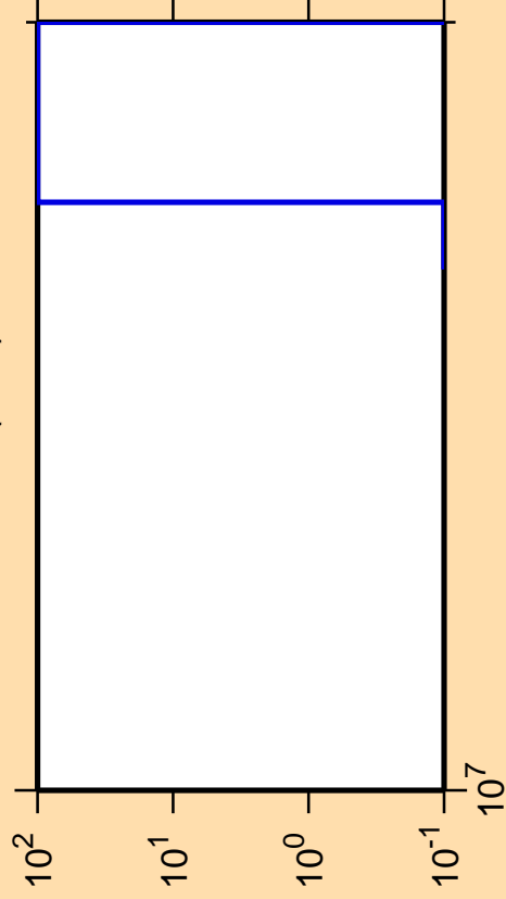
\Delta\sigma/\sigma vs. E for ^{132}\text{Ba}(n,nt)
