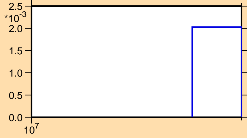
\sigma vs. E for ^{132}\text{Ba}(n,3n)
