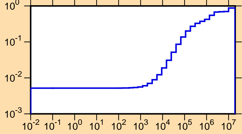
\mu vs. E for ^{132}\text{Ba}(\text{mt251})
