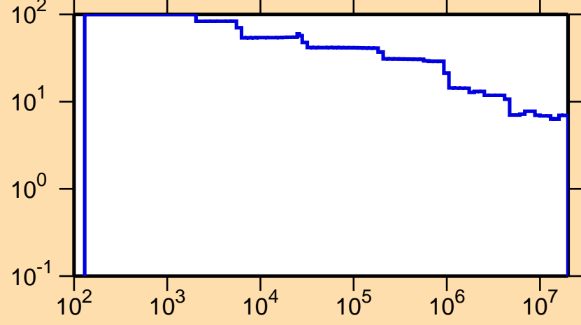
\Delta\sigma/\sigma vs. E for ^{133}\text{Ba}(n,\text{nonel.})
