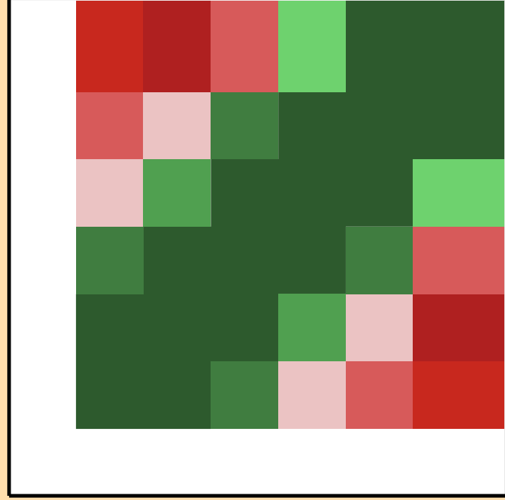
\sigma vs. E for ^{133}\text{Ba}(n,n_{\text{cont}}) .
