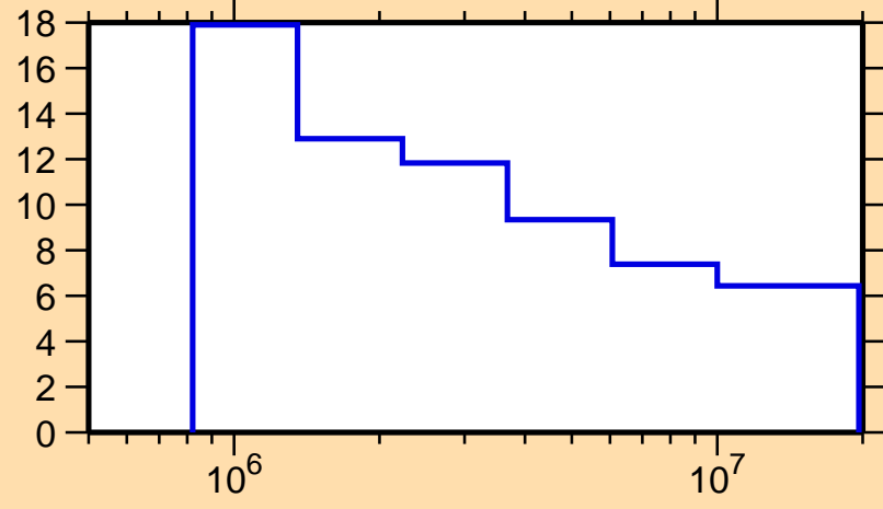
\Delta\sigma/\sigma vs. E for ^{133}\text{Ba}(n,n\text{nonel.})
