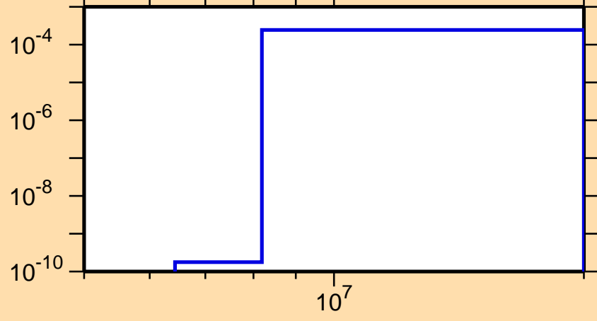
\sigma vs. E for ^{133}\text{Ba}(n,n\alpha)
