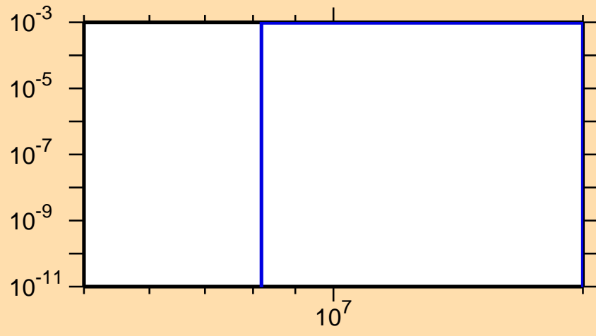
\sigma vs. E for ^{133}\text{Ba}(n,d)
