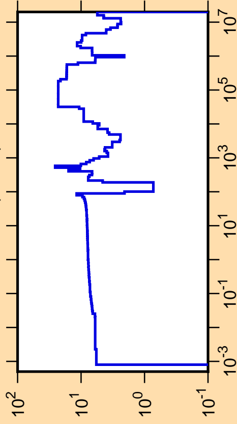
\Delta\sigma/\sigma vs. E for ^{134}\text{Ba}(n,\text{tot.})
