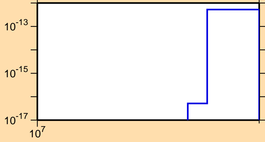
\sigma vs. E for ^{134}\text{Ba}(n,\text{pd})
