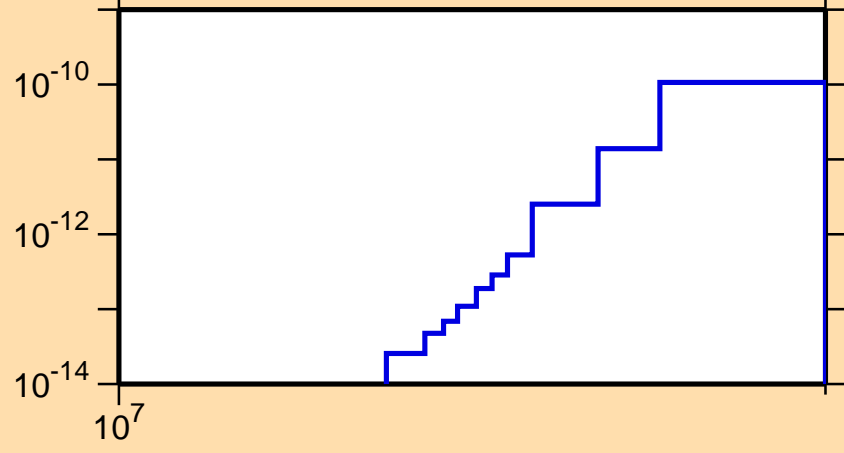
\sigma vs. E for ^{135}\text{Ba}(n,p\alpha)
