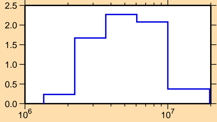
\sigma vs. E for ^{135}\text{Ba}(n,n\text{cont.})
