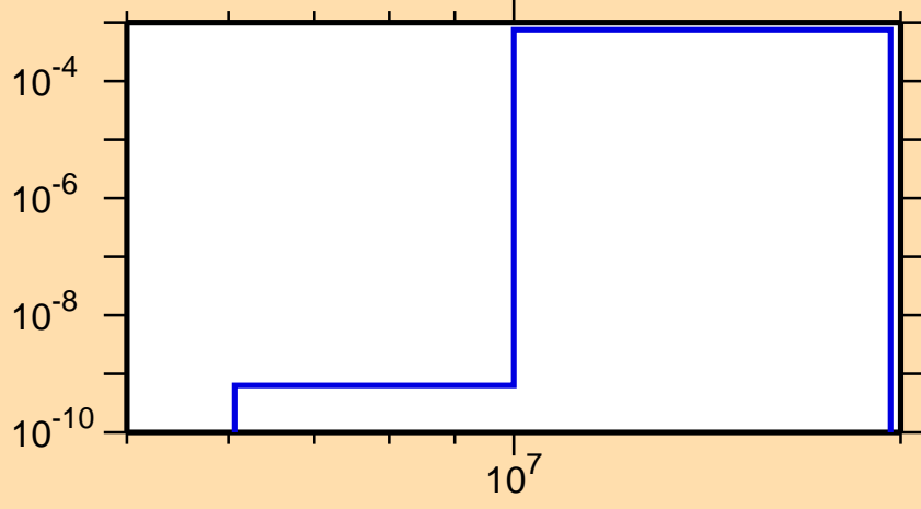
\sigma vs. E for ^{135}\text{Ba}(n,d)
