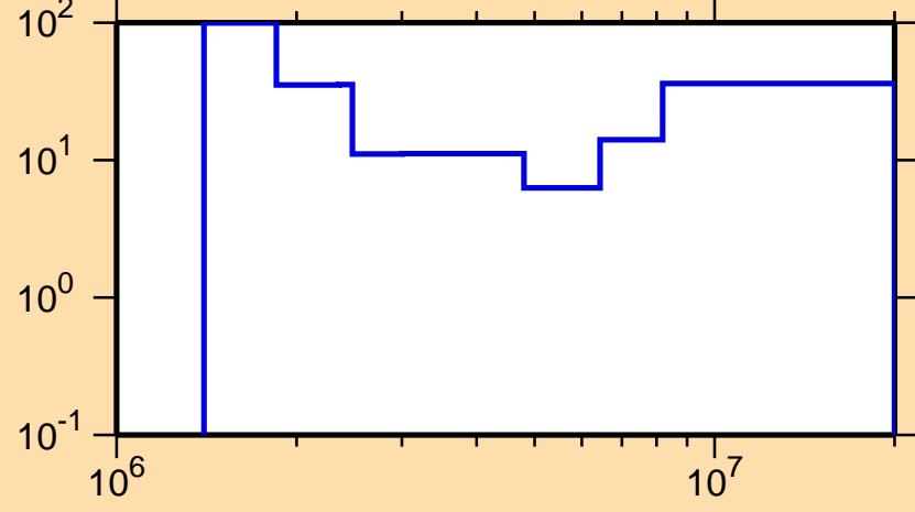
\Delta\sigma/\sigma vs. E for ^{135}\text{Ba}(n,n\text{cont.})
