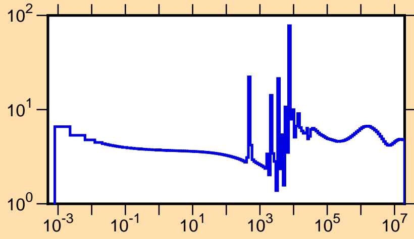
\sigma vs. E for ^{136}\text{Ba}(n,\text{tot.})
