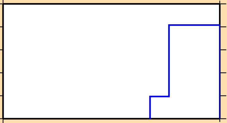
\sigma vs. E for ^{136}\text{Ba}(n,2n\alpha)
