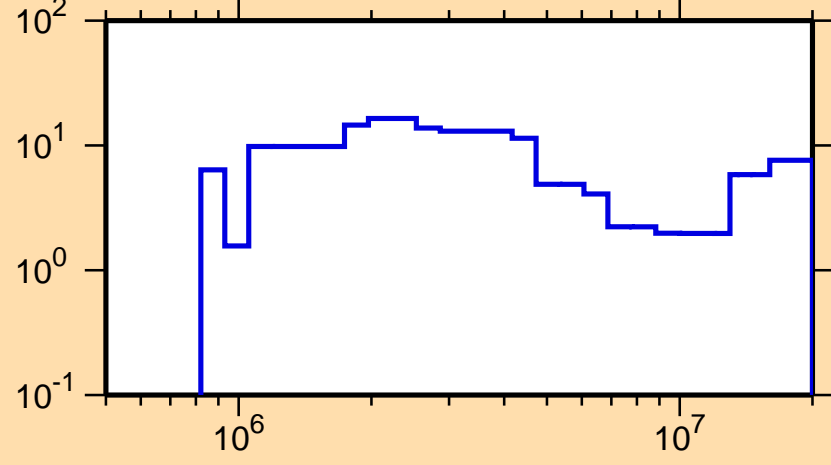
\Delta\sigma/\sigma vs. E for ^{136}\text{Ba}(n,\text{tot.})
