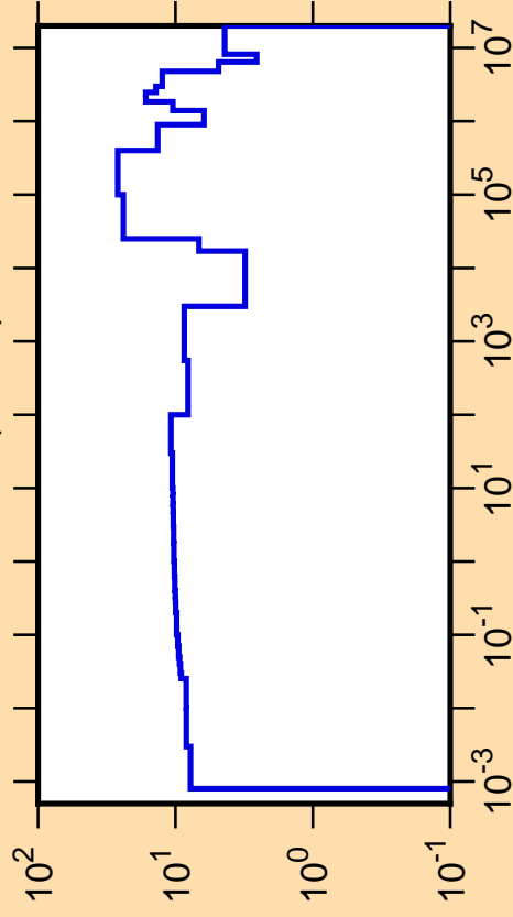
\Delta\sigma/\sigma vs. E for ^{136}\text{Ba}(n,\text{tot.})
