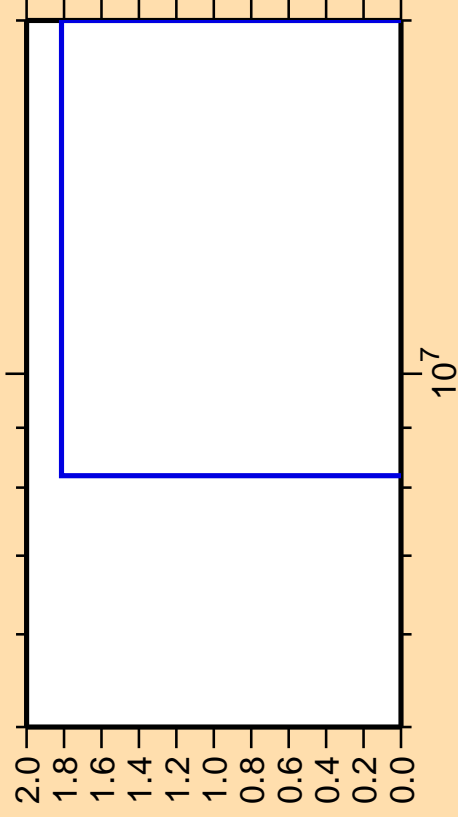
\Delta\sigma/\sigma vs. E for ^{136}\text{Ba}(n,nt)
