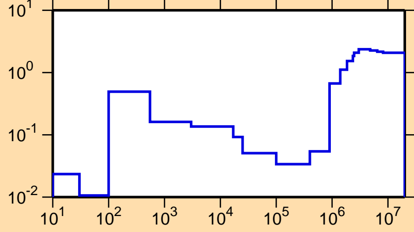
\sigma vs. E for ^{136}\text{Ba}(n,\text{nonel.})
