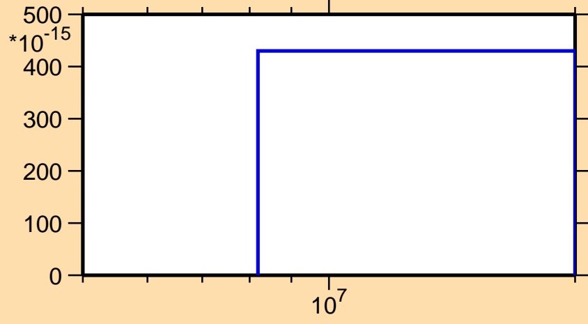
\sigma vs. E for ^{136}\text{Ba}(n,nt)
