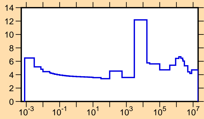
\sigma vs. E for ^{136}\text{Ba}(n,\text{tot.})
