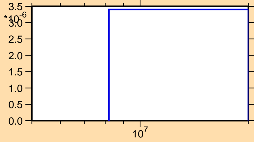
\sigma vs. E for ^{136}\text{Ba}(n,t)
