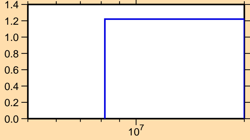
\sigma vs. E for ^{136}\text{Ba}(n,2n)
