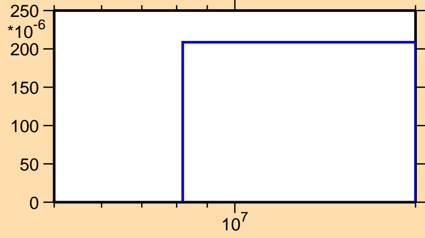
\sigma vs. E for ^{136}\text{Ba}(n,np)
