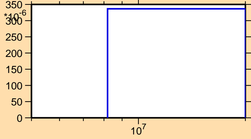
\sigma vs. E for ^{136}\text{Ba}(n,d)
