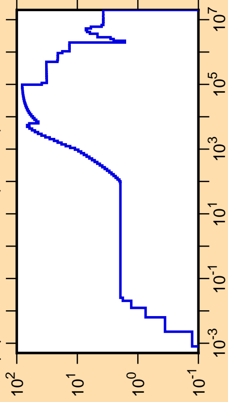
\Delta\mu/\mu vs. E for ^{137}\text{Ba}(\text{mt251})
