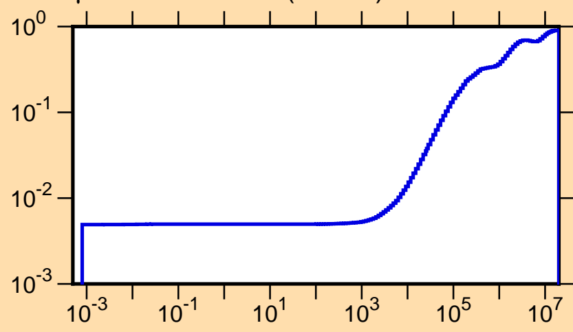
\mu vs. E for ^{137}\text{Ba}(\text{mt251})
