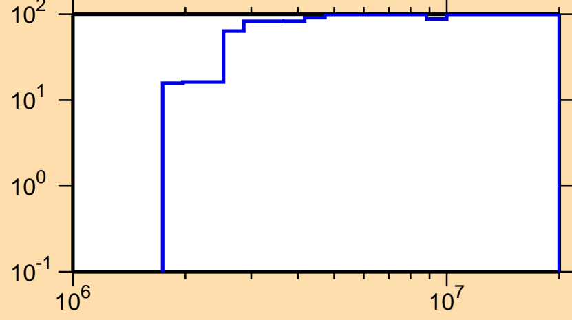
\Delta\sigma/\sigma vs. E for ^{137}\text{Ba}(n,\gamma)
