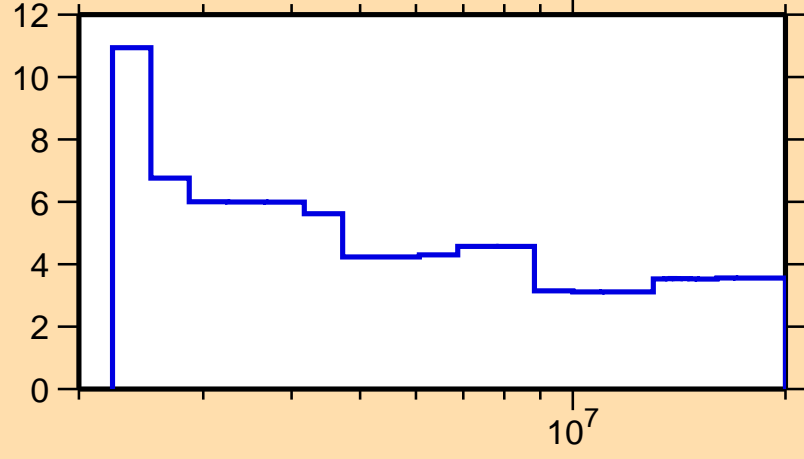
\Delta\sigma/\sigma vs. E for ^{137}\text{Ba}(n,n_{\text{inel}}) .
