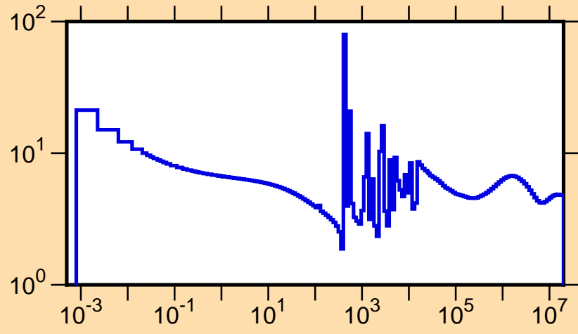
\sigma vs. E for ^{137}\text{Ba}(n,\text{tot.})
