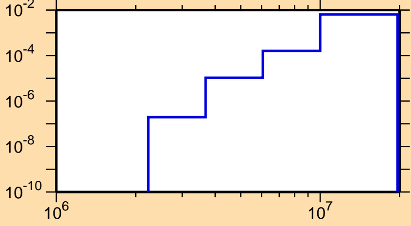
\sigma vs. E for ^{137}\text{Ba}(n,p)
