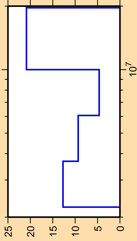
\Delta\sigma/\sigma vs. E for ^{137}\text{Ba}(n,ncont.)
