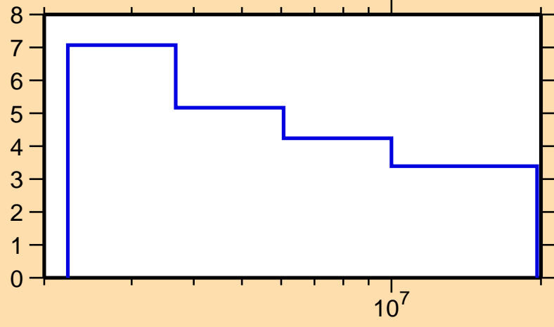
\Delta\sigma/\sigma vs. E for ^{137}\text{Ba}(n,n\text{nonel.})
