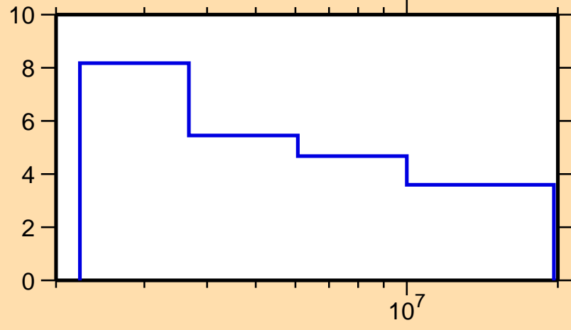
\Delta\sigma/\sigma vs. E for ^{137}\text{Ba}(n,el.)
