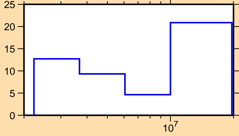
\Delta\sigma/\sigma vs. E for ^{137}\text{Ba}(n,ncont.)
