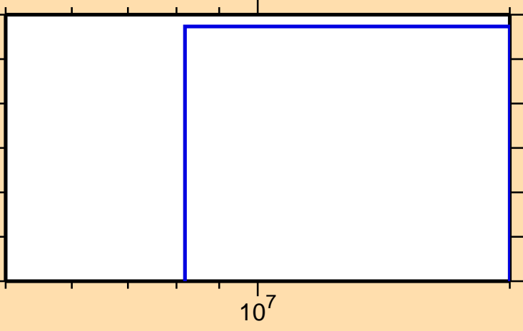
\sigma vs. E for ^{137}\text{Ba}(n,\text{nd})
