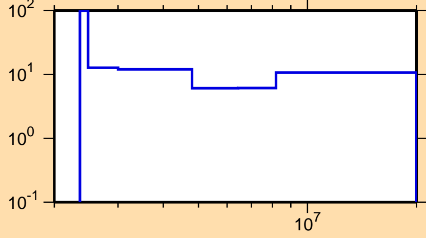
\Delta\sigma/\sigma vs. E for ^{137}\text{Ba}(n,ncont.)
