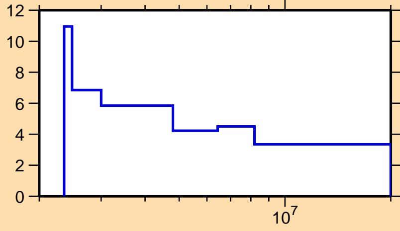
\Delta\sigma/\sigma vs. E for ^{137}\text{Ba}(n,n\text{onel.})
