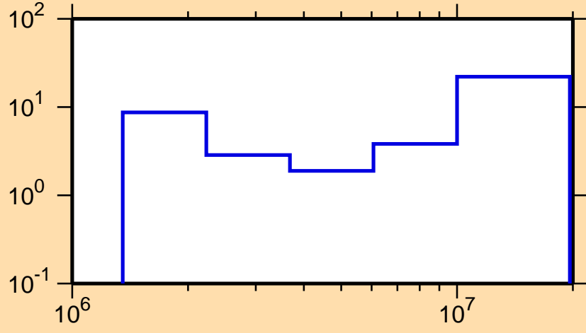
\Delta\sigma/\sigma vs. E for ^{137}\text{Ba}(n,n\text{cont.})
