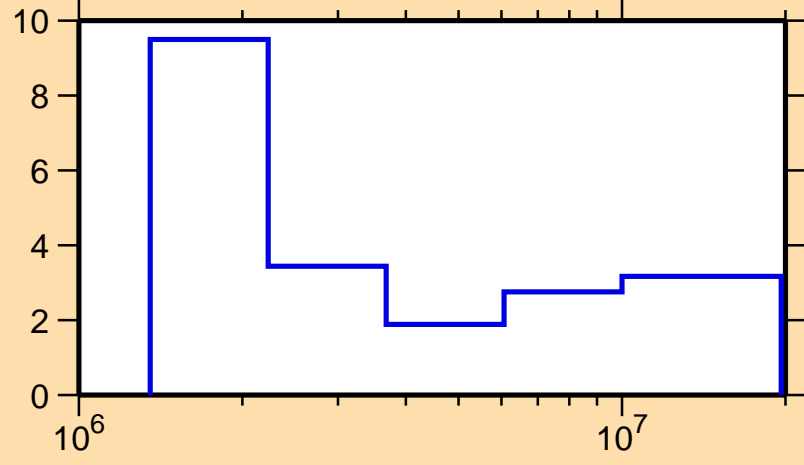
\Delta\sigma/\sigma vs. E for ^{137}\text{Ba}(n,n\text{nonel.})
