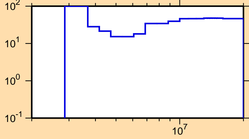
\Delta\sigma/\sigma vs. E for ^{140}\text{Ba}(n,n\text{cont.})
