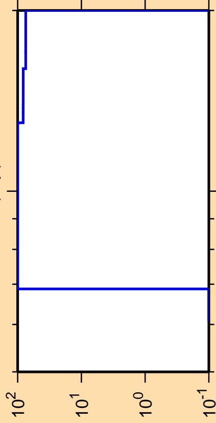
\Delta\sigma/\sigma vs. E for ^{140}\text{Ba}(n,p)
