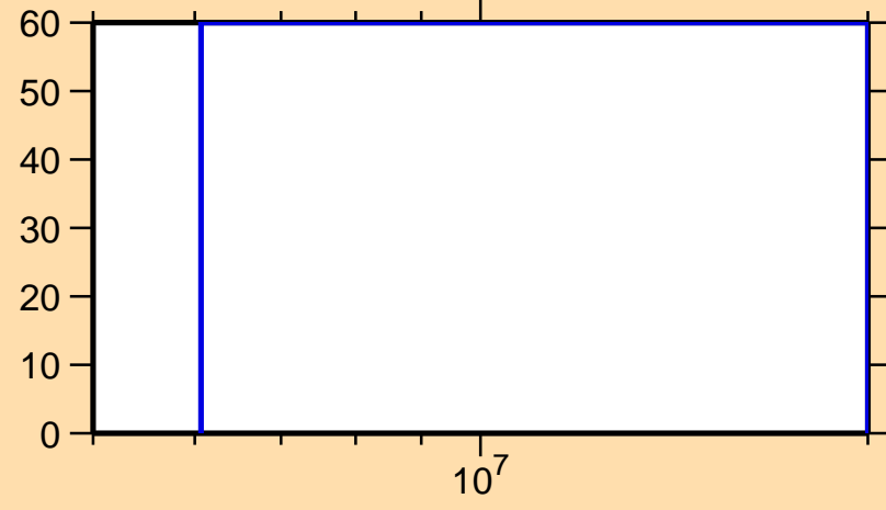
\Delta\sigma/\sigma vs. E for ^{140}\text{Ba}(n,\gamma)
