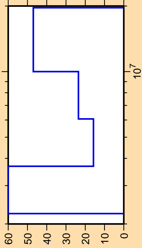
\Delta\sigma/\sigma vs. E for ^{140}\text{Ba}(n,ncont.)
