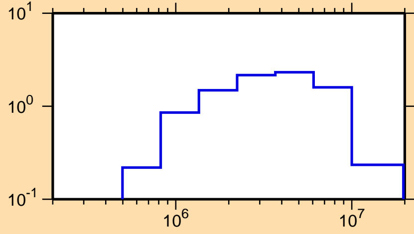
\sigma vs. E for ^{140}\text{Ba}(n,\text{inel.})
