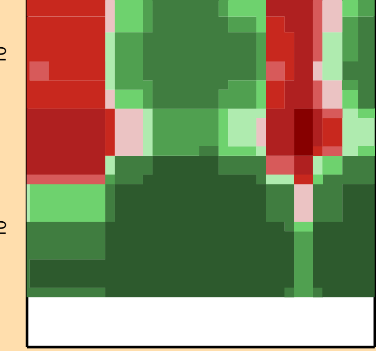
Correlation Matrix
