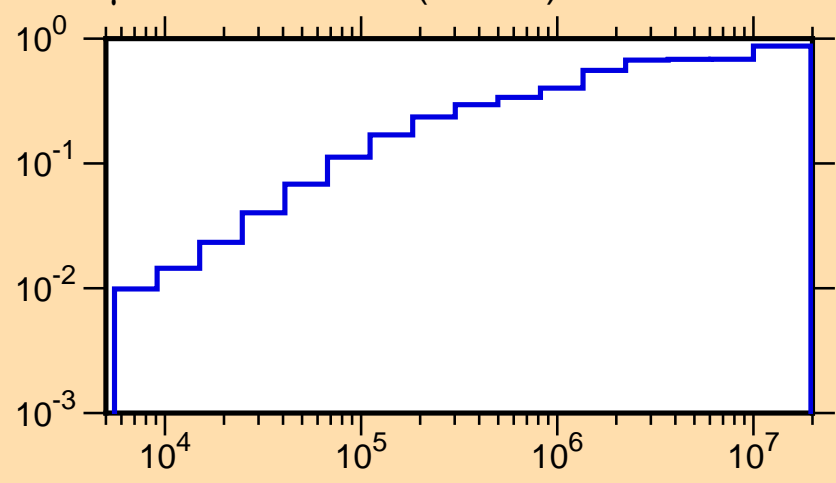
\mu vs. E for ^{142}\text{Ba}(\text{mt251})
