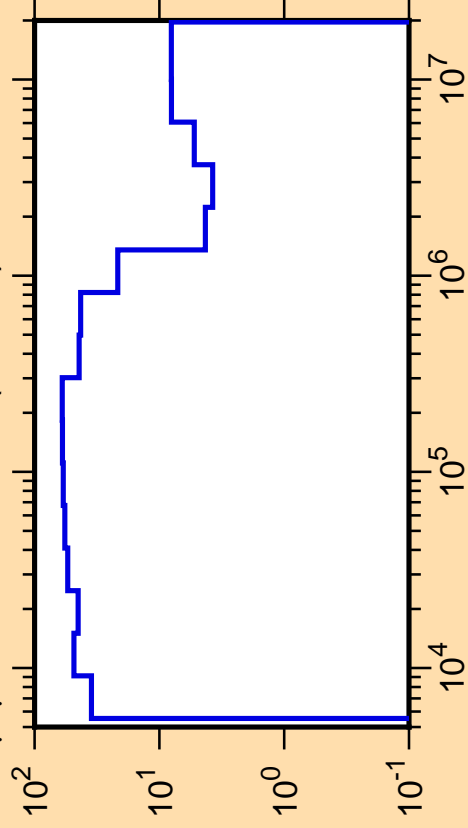
\Delta\mu/\mu vs. E for ^{142}\text{Ba}(\text{mt251})
