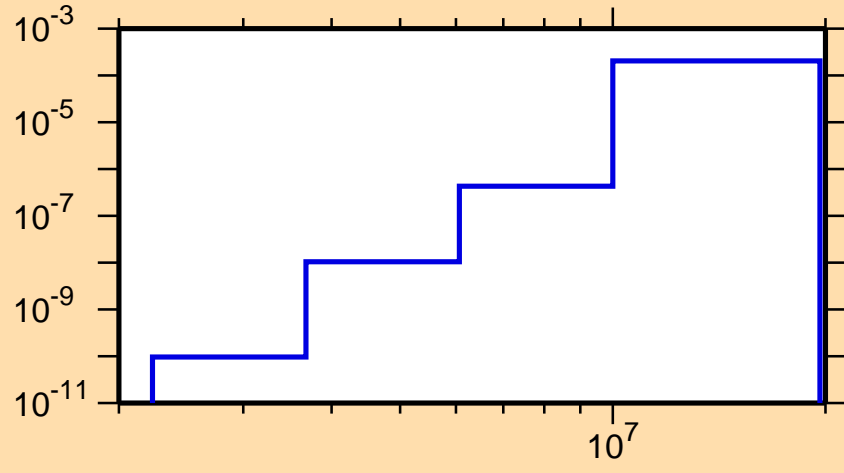
\sigma vs. E for ^{142}\text{Ba}(n,\alpha)
