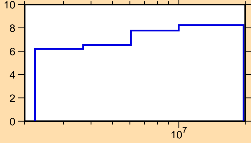
\Delta\sigma/\sigma vs. E for ^{142}\text{Ba}(n,n\text{nonel.})
