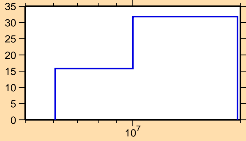
\Delta\sigma/\sigma vs. E for ^{142}\text{Ba}(n,ncont.)
