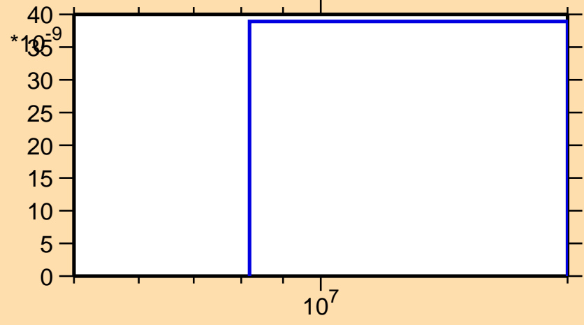
\sigma vs. E for ^{142}\text{Ba}(n,\text{nt})
