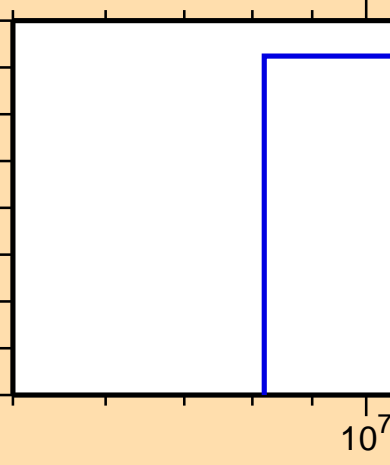
\sigma vs. E for ^{142}\text{Ba}(n,np)
