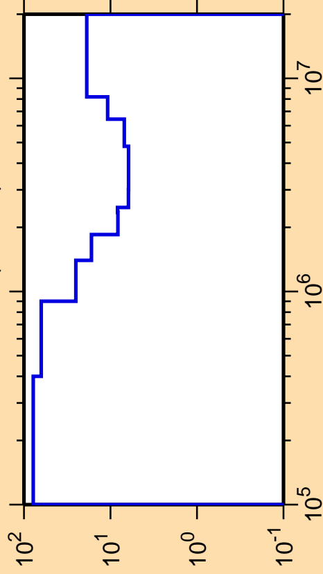
\Delta\sigma/\sigma vs. E for ^{142}\text{Ba}(n,\text{inel.})
