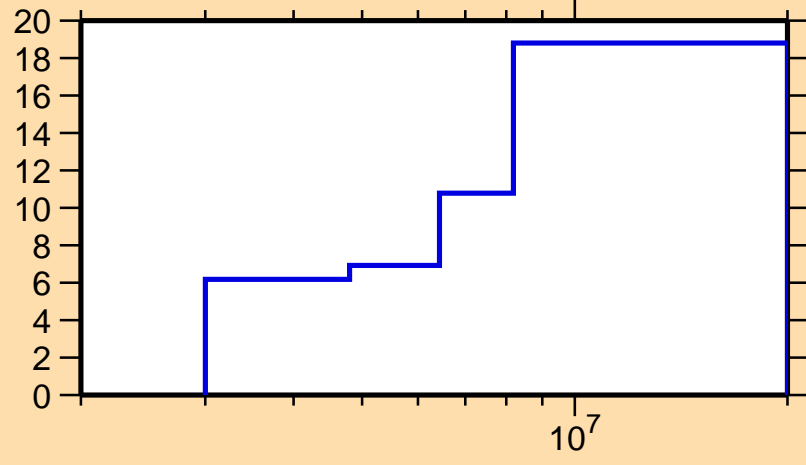
\Delta\sigma/\sigma vs. E for ^{142}\text{Ba}(n,inel.)
