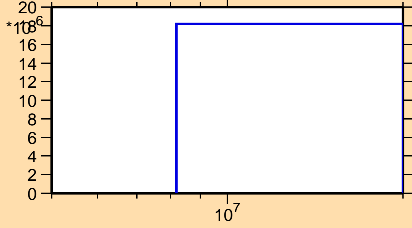
\sigma vs. E for ^{142}\text{Ba}(n,t)
