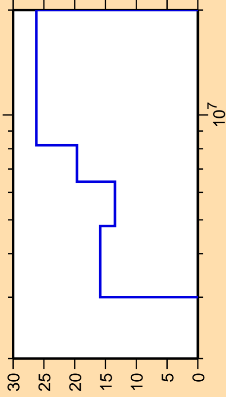
\Delta\sigma/\sigma vs. E for ^{142}\text{Ba}(n,ncont.)
