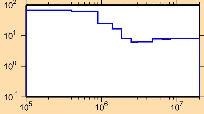
\Delta\sigma/\sigma vs. E for ^{142}\text{Ba}(n,\text{nonel.})
