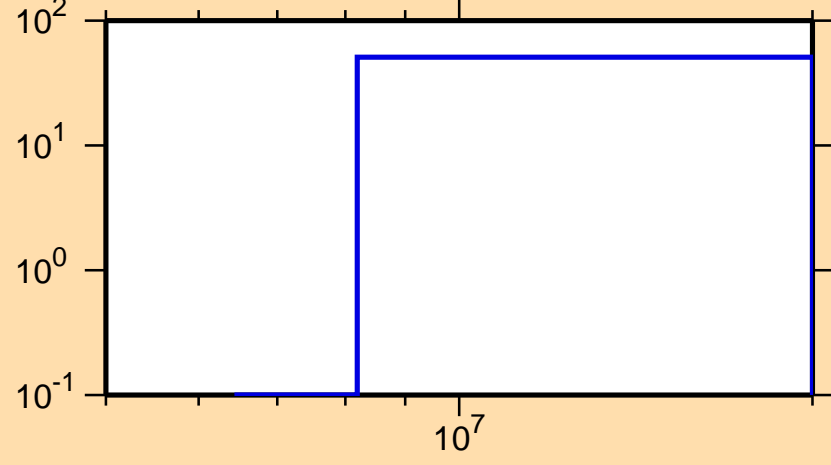
\Delta\sigma/\sigma vs. E for ^{142}\text{Ba}(n,p)
