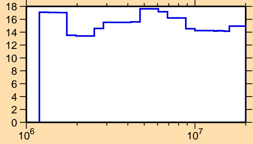
\Delta\sigma/\sigma vs. E for ^{143}\text{Ba}(n,n\text{onel.})
