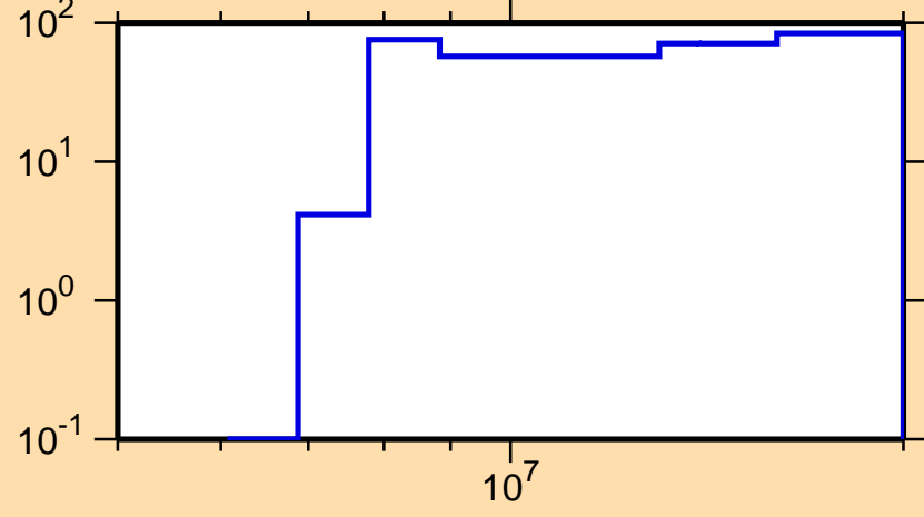
\Delta\sigma/\sigma vs. E for ^{143}\text{Ba}(n,p)
