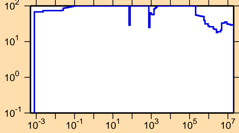
\Delta\sigma/\sigma vs. E for ^{143}\text{Ba}(n,\text{tot.})
