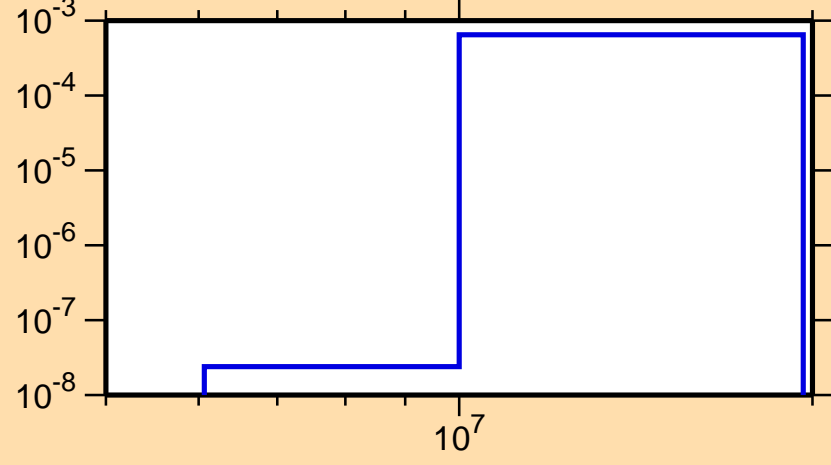
\sigma vs. E for ^{143}\text{Ba}(n,p)
