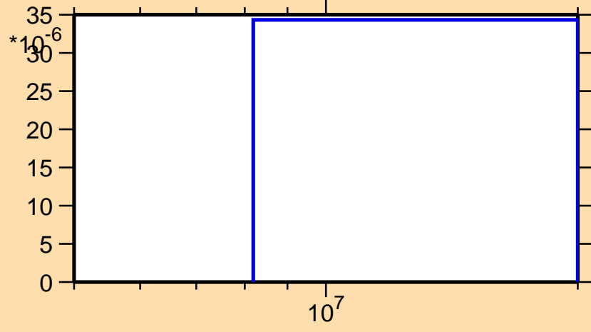
\sigma vs. E for ^{143}\text{Ba}(n,d)
