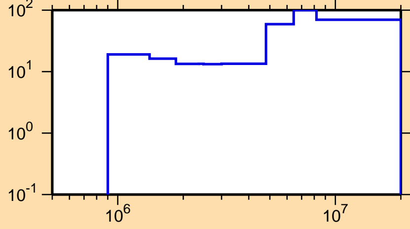
\Delta\sigma/\sigma vs. E for ^{143}\text{Ba}(n,\text{inel.})
