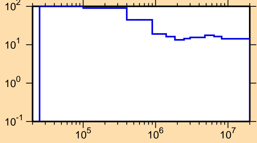
\Delta\sigma/\sigma vs. E for ^{143}\text{Ba}(n,\text{nonel.})
