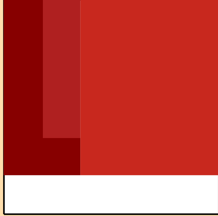
\Delta\sigma/\sigma vs. E for ^{143}\text{Ba}(n,\text{el.})
