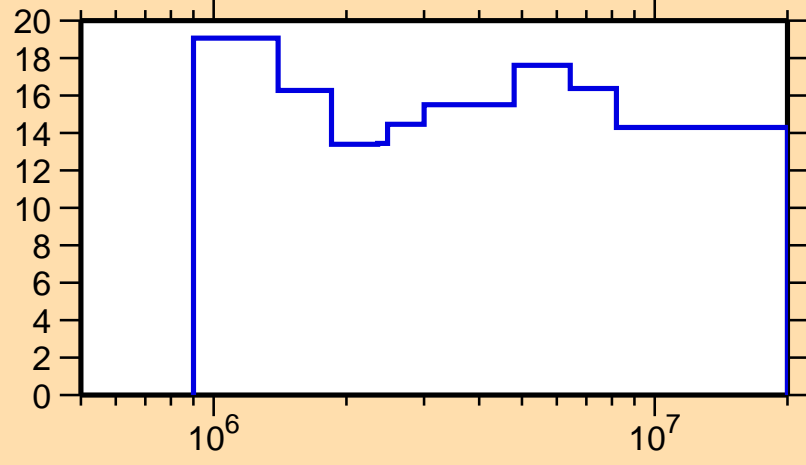
\Delta\sigma/\sigma vs. E for ^{143}\text{Ba}(n,n\text{nonel.})
