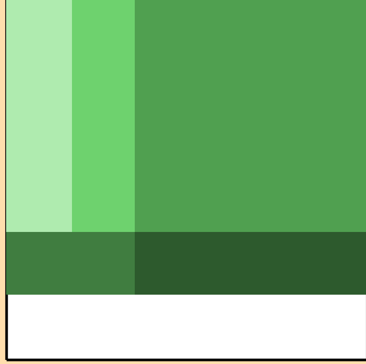
\Delta\sigma/\sigma vs. E for ^{143}\text{Ba}(n,n_1)
