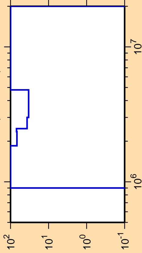
\Delta\sigma/\sigma vs. E for ^{143}\text{Ba}(n,\text{ncont.})
