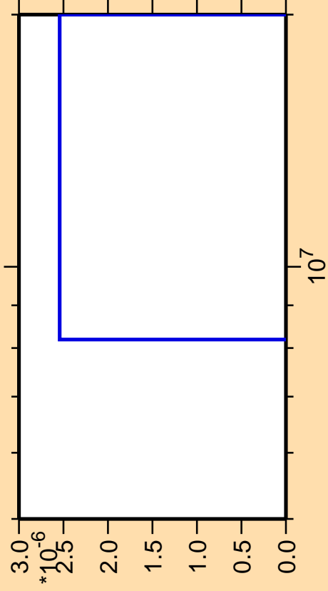
\Delta\sigma/\sigma vs. E for ^{143}\text{Ba}(\text{mt } 11)
