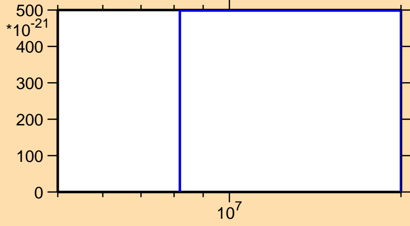
\sigma vs. E for ^{143}\text{Ba}(\text{mt } 11)
