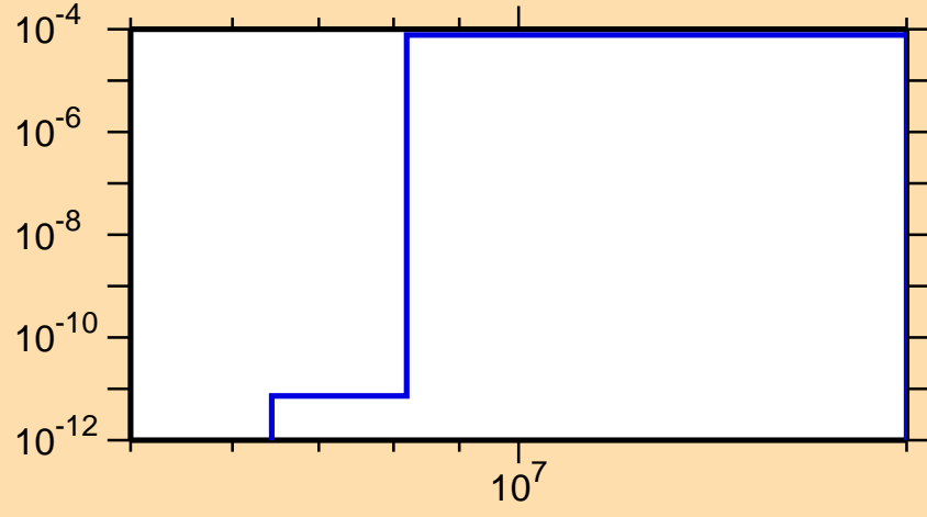
\sigma vs. E for ^{143}\text{Ba}(n,n\alpha)
