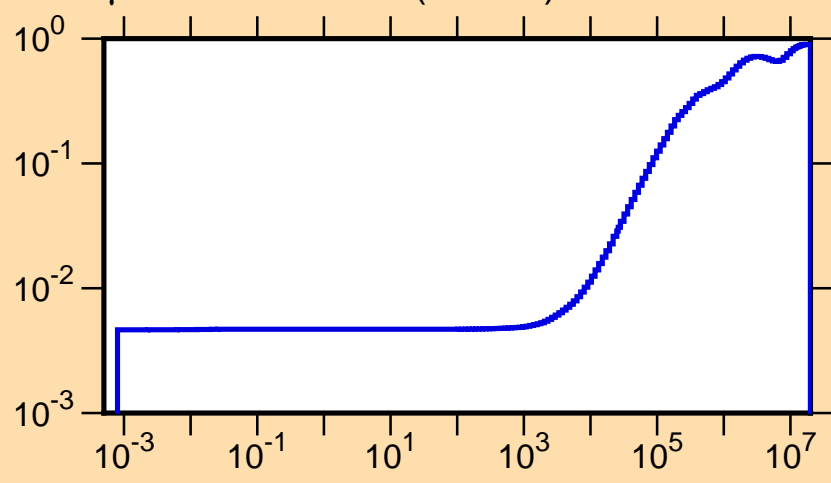
\mu vs. E for ^{145}\text{Ba}(\text{mt251})
