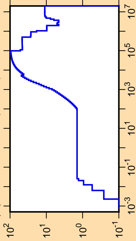
\Delta\mu/\mu vs. E for ^{145}\text{Ba}(\text{mt251})
