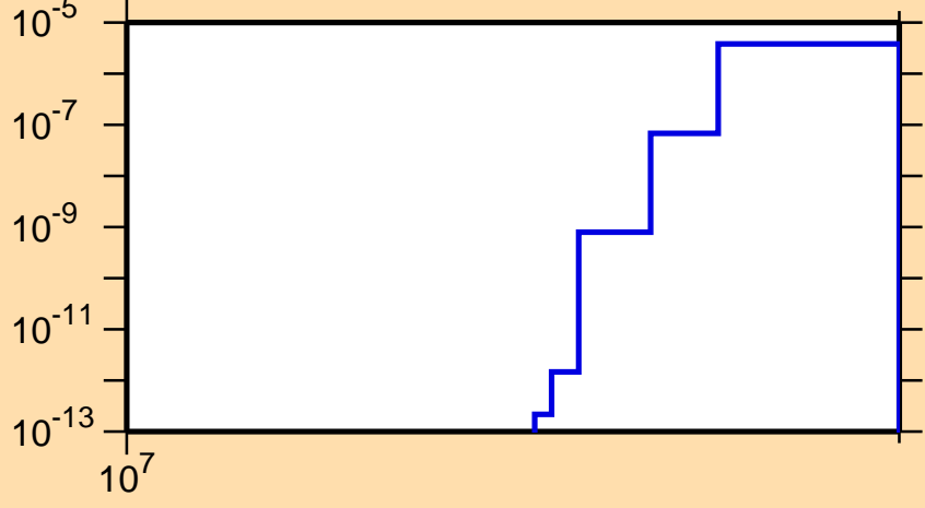
\sigma vs. E for ^{145}\text{Ba}(n,nt)
