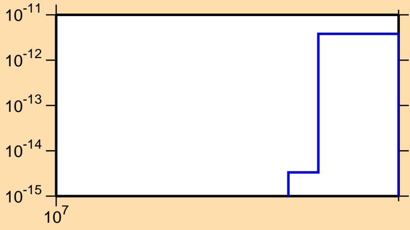
\sigma vs. E for ^{145}\text{Ba}(n,3n\alpha)
