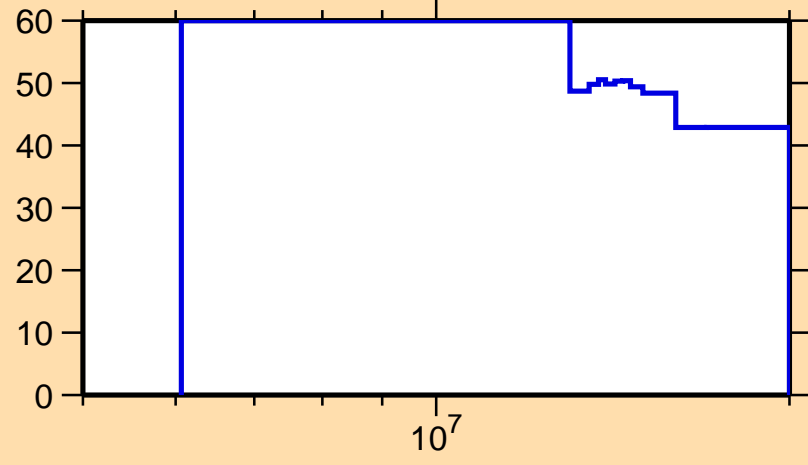
\Delta\sigma/\sigma vs. E for ^{145}\text{Ba}(n,n\text{cont.})
