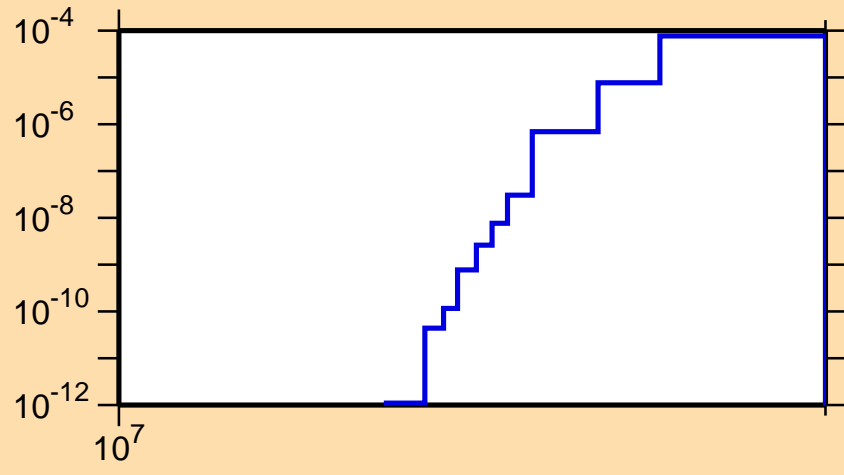
\sigma vs. E for ^{145}\text{Ba}(n,np)
