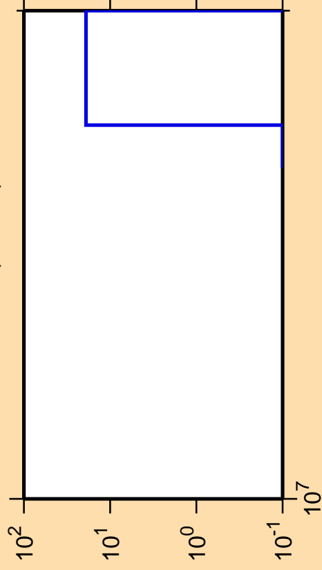
\Delta\sigma/\sigma vs. E for ^{145}\text{Ba}(n,3n\alpha)
