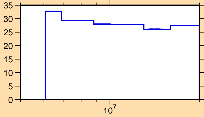
\Delta\sigma/\sigma vs. E for ^{145}\text{Ba}(n,n_1)
